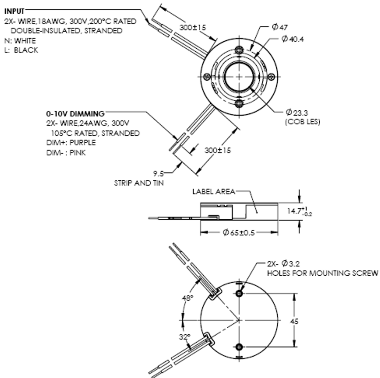
Figure 8c: Mechanical Drawing (Double Insulation)
