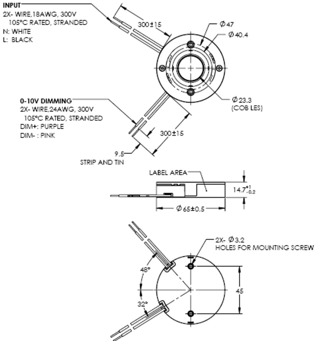
Figure 8b: Mechanical Drawing (Loose wires)
