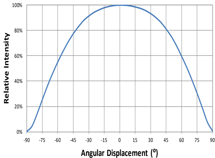
Figure 5: Typical Spatial Radiation Pattern at 150mA, T_{sp}=25^{\circ}\text{C}
