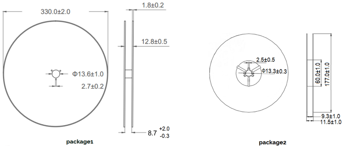
Figure 10: Emitter Reel Drawings
