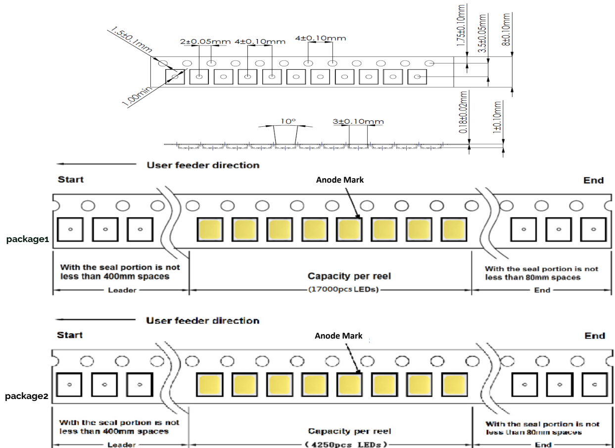
Figure 11: Emitter Tape Drawings
