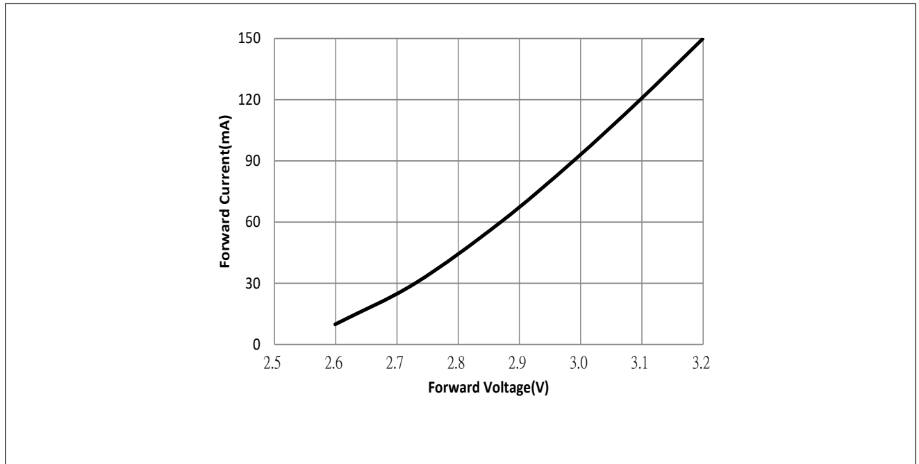
Figure 1: Drive Current vs. Forward Voltage ( T_{sp}=25^{\circ}\text{C} )
