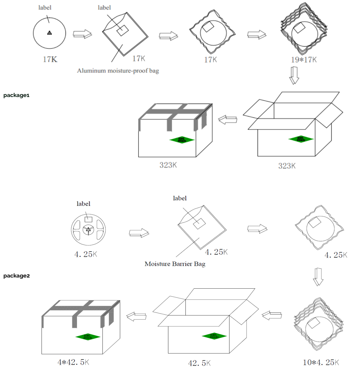
Figure 12: Emitter Reel Packaging Drawings
