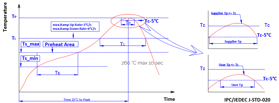
Figure 9 : Reflow Profile (Reflow frequency 2 times max)
