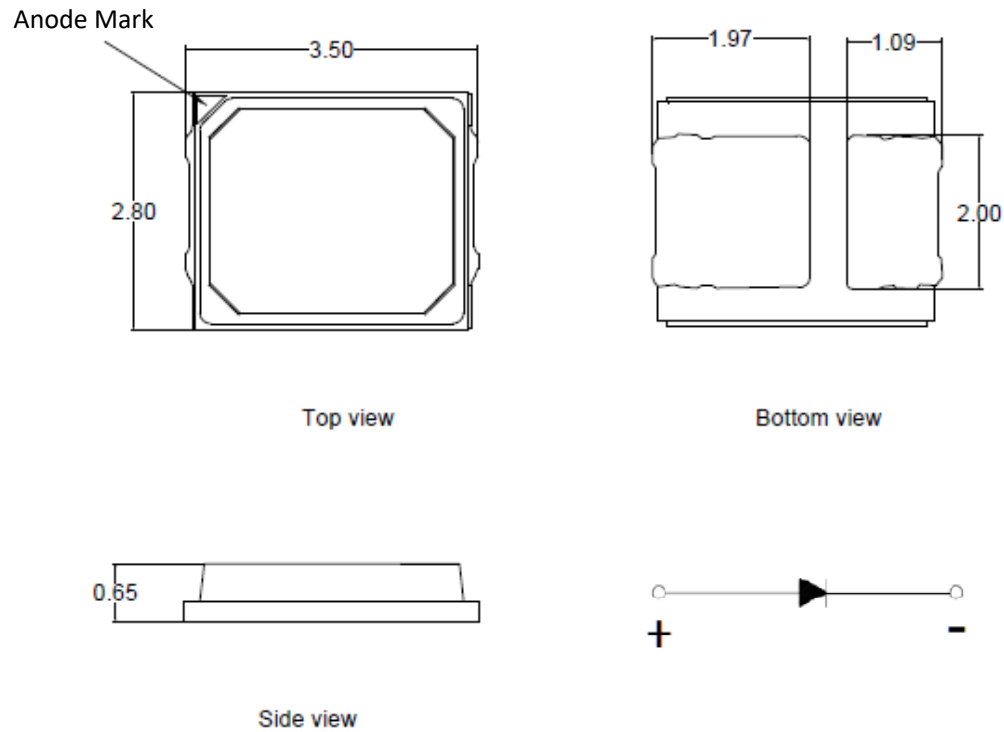
Figure 8: Drawing for SMD 2835
