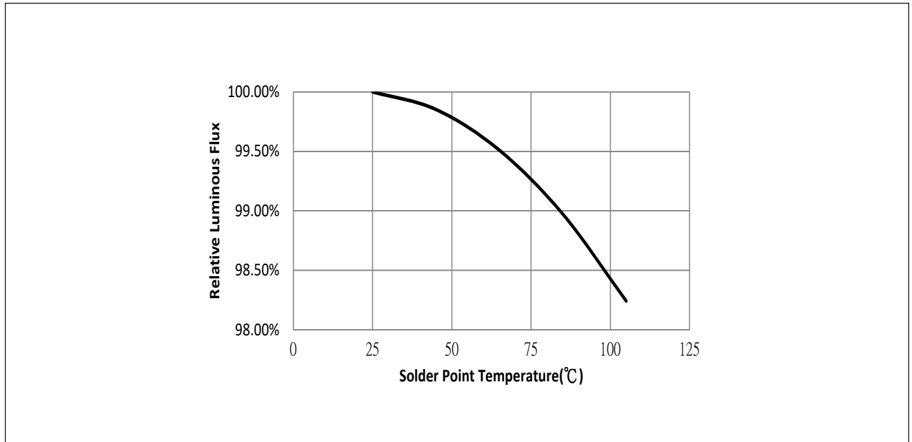
Figure 3: Relative Flux vs. Solder Point Temperature
