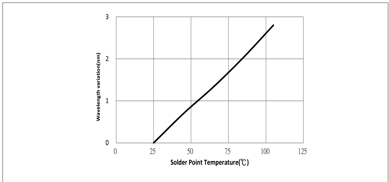
Figure 4: Relative Wavelength variation vs. Temperature
