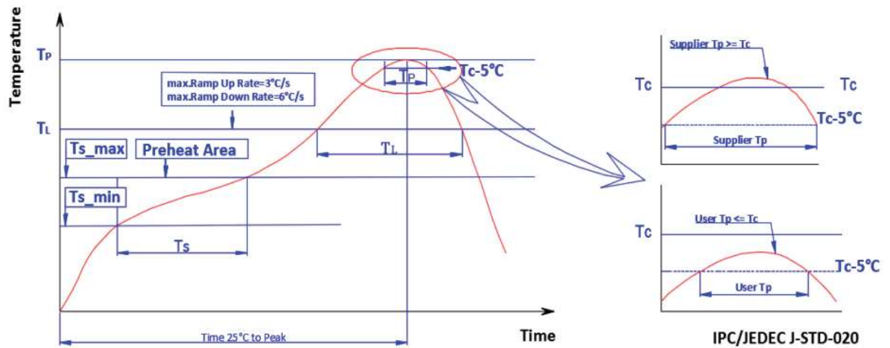
Figure 12 : Reflow Profile
