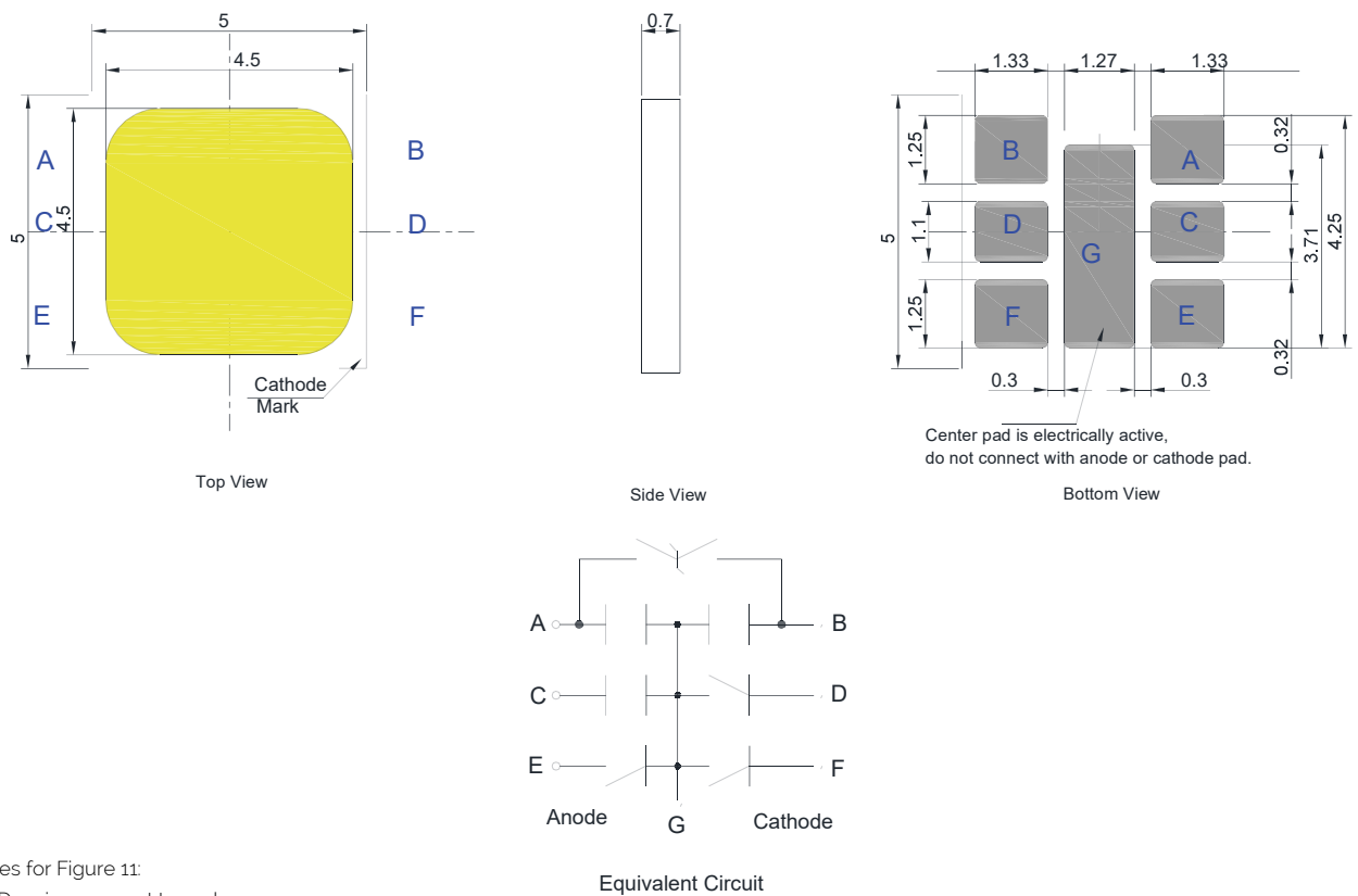
Figure 11: Drawing for SMD 5050
