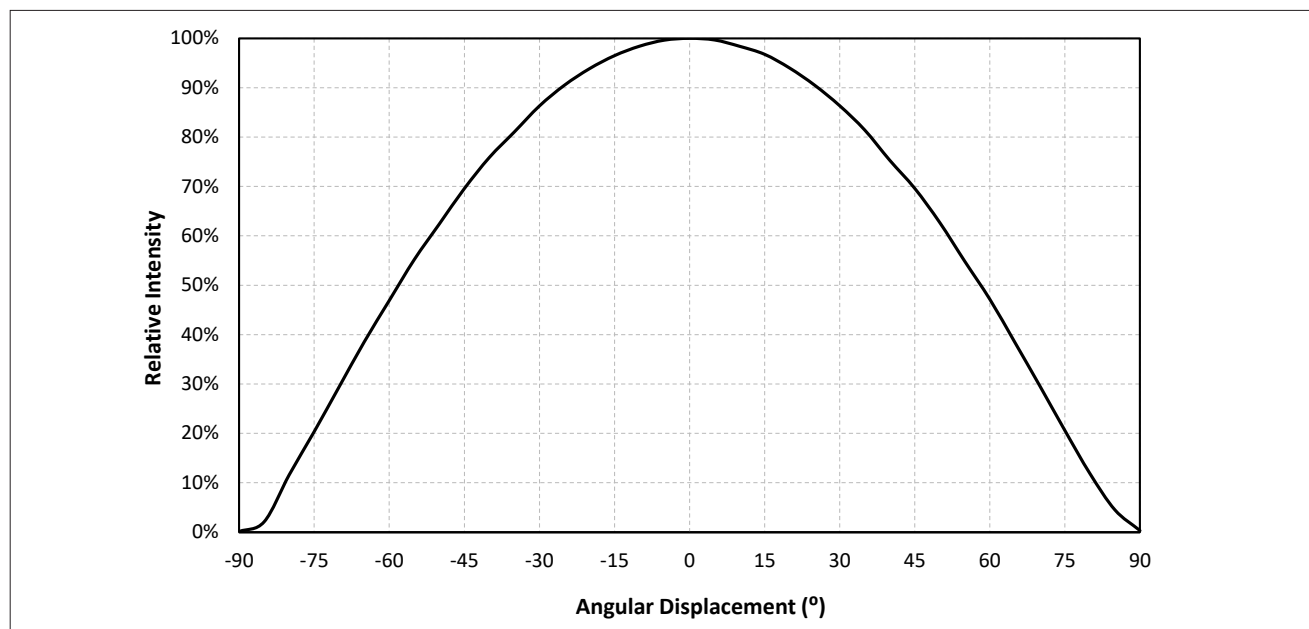
Figure 8: Typical Spatial Radiation Pattern at 350mA, T_{sp}=25^{\circ}\text{C}
