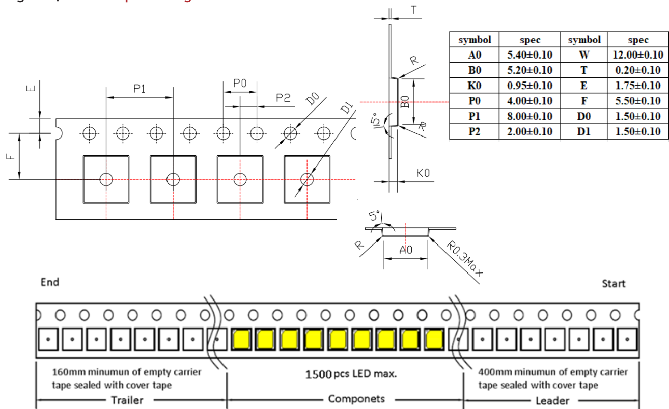
Figure 14: Emitter Tape Drawings
