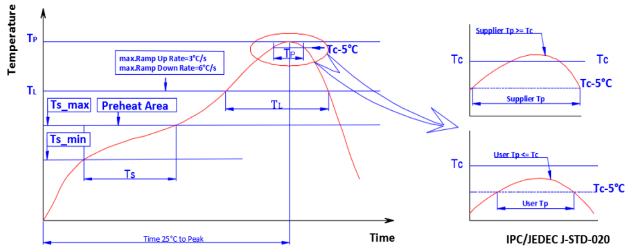
Figure 12 : Reflow Profile
