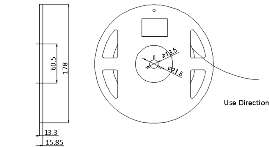
Figure 13: Emitter Reel Drawings
