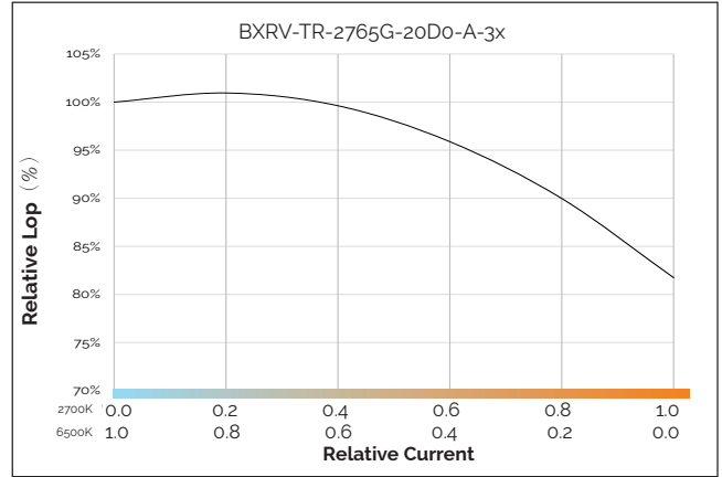
Figure 8: Relative Flux vs. Relative Current
