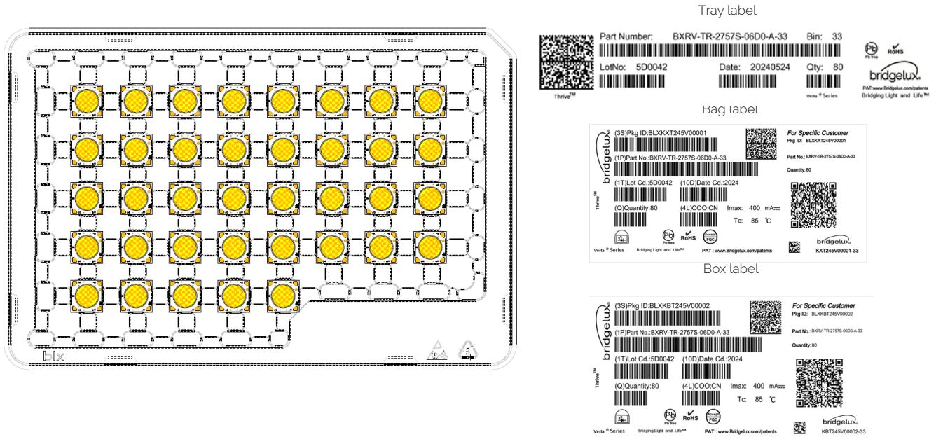
Figure 21: Vesta Series Tunable White 9mm Packaging and Labeling
