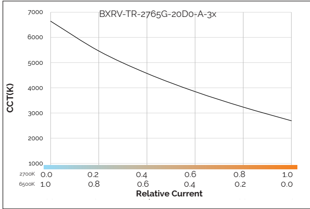
Figure 7: CCT vs. Relative Current
