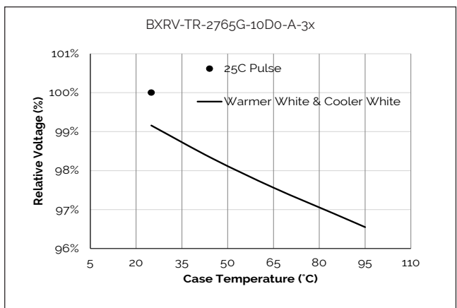
Figure 10: Relative Voltage vs. Case Temperature
