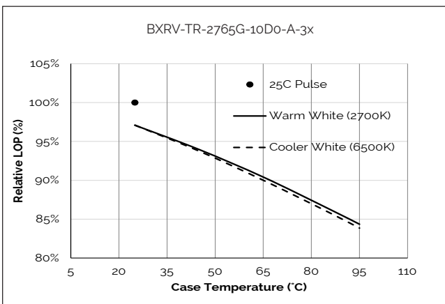
Figure 9: Relative Flux vs. Case Temperature
