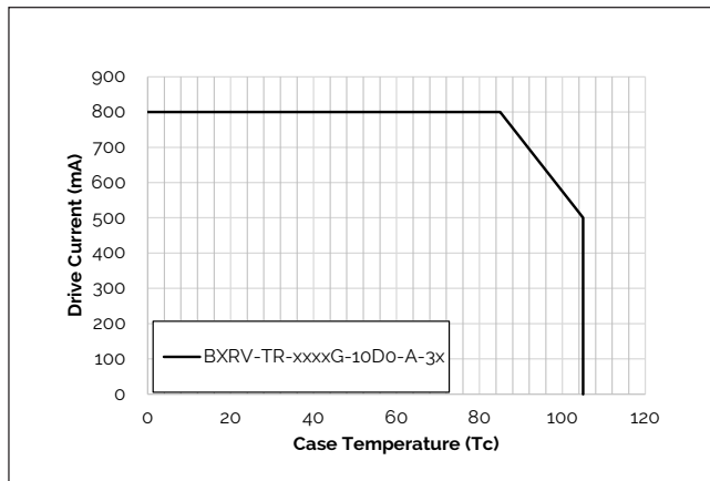
Figure 14: Derating Curve
