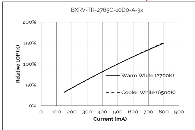
Figure 8: Relative Flux vs. Drive Current, T_c=25^\circ\text{C}
