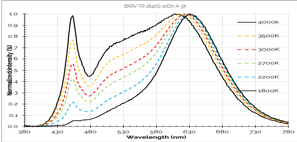
Figure 17: 1800K-4000K with CRI90
