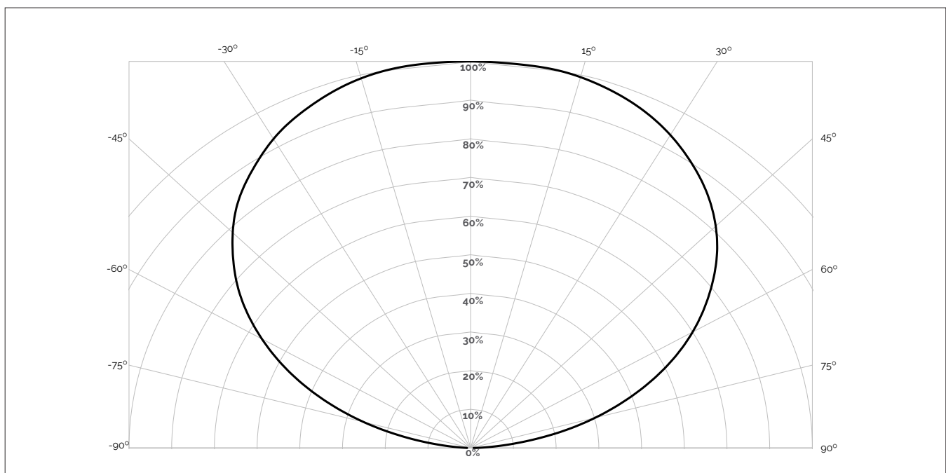
Figure 16: Typical Polar Radiation Pattern
