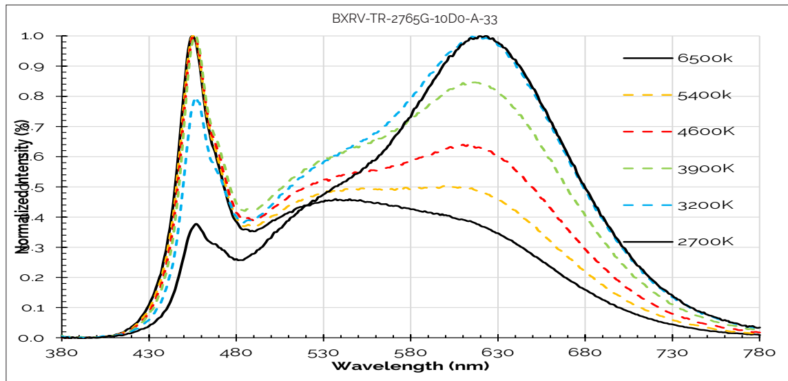
Figure 18: 2700K - 6500K with 90 CRI
