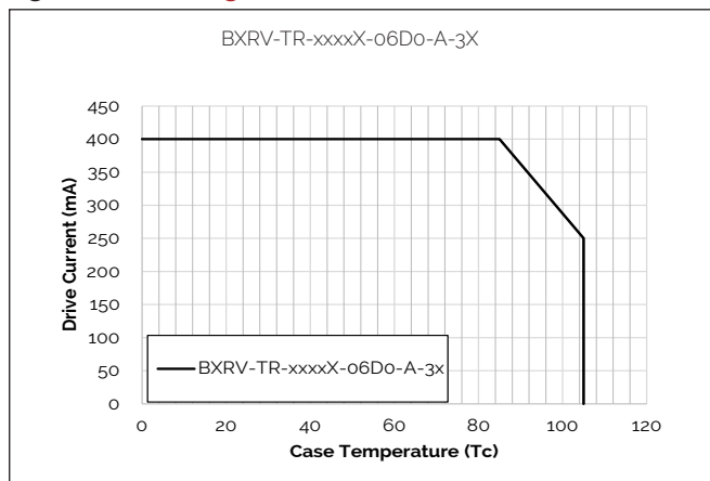
Figure 15: Derating Curve
