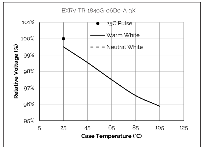
Figure 4: Relative Voltage vs. Case Temperature
