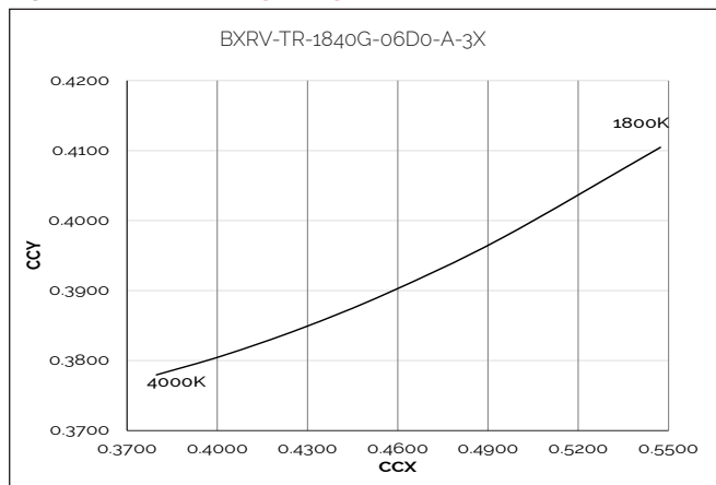
Figure 13: CCT Tuning Range, Tc=85°C
