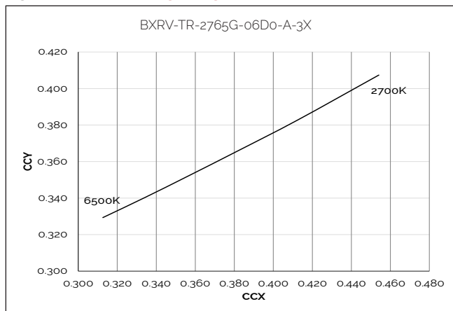
Figure 14: CCT Tuning Range, Tc=85°C
