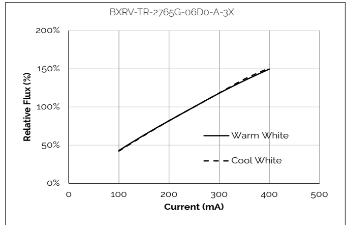
Figure 8: Relative Flux vs. Drive Current, T_c=25^\circ\text{C}
