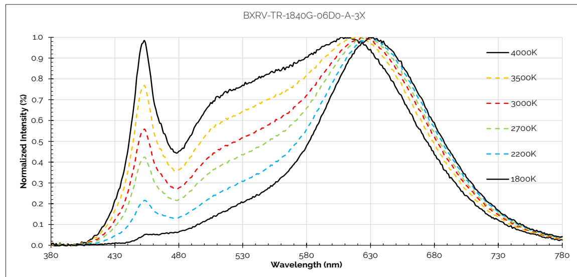
Figure 18: 1800K-4000K with CRI90
