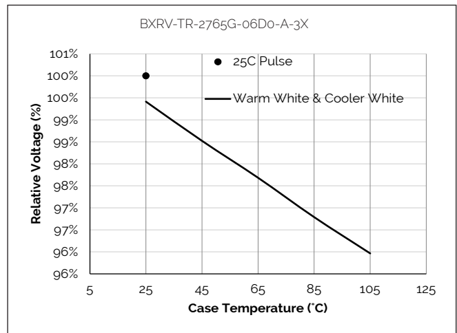
Figure 10: Relative Voltage vs. Case Temperature
