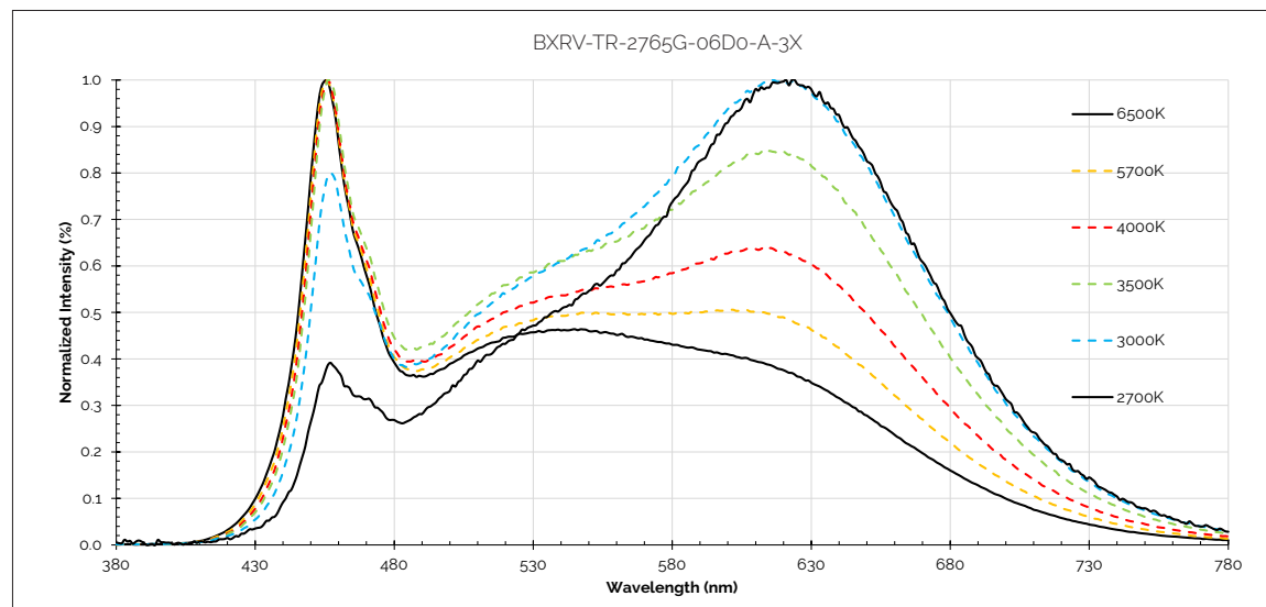
Figure 19: 2700K-6500K with CRI90
