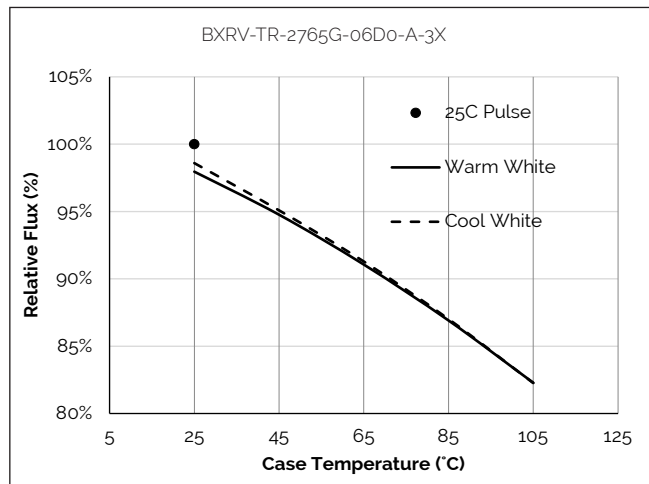
Figure 9: Relative Flux vs. Case Temperature
