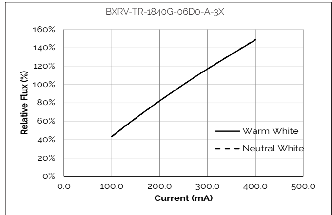
Figure 2: Relative Flux vs. Drive Current, T_c = 25^\circ\text{C}
