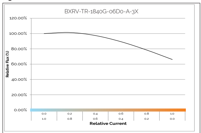
Figure 6: Relative Flux vs. Relative Current
