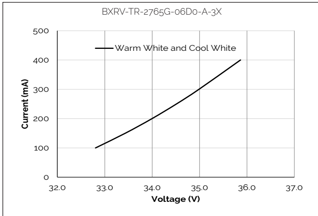
Figure 7: Forward Voltage vs. Forward Current, T_c=25^\circ\text{C}
