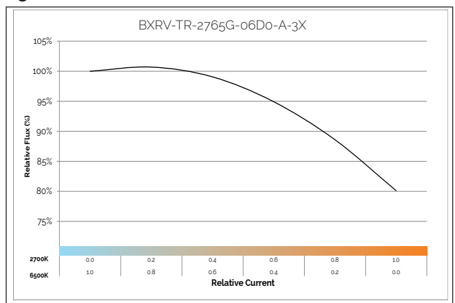
Figure 12: Relative Flux vs. Relative Current
