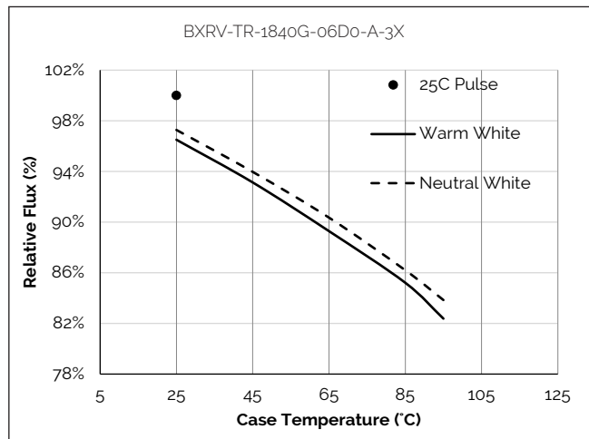
Figure 3: Relative Flux vs. Case Temperature
