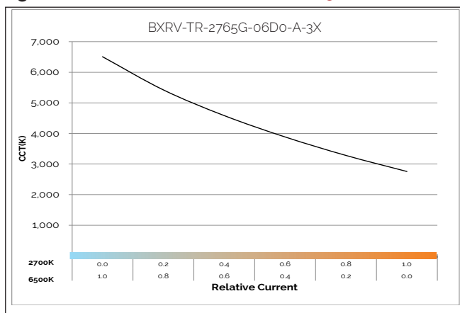
Figure 11: CCT vs. Relative Current, T_c=85^\circ\text{C}
