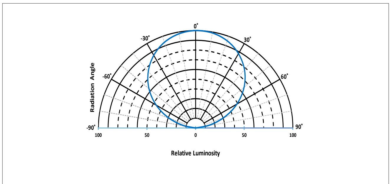
Figure 8: Typical Polar Radiation Pattern at 20mA, T_{sp}=25^{\circ}\text{C}
