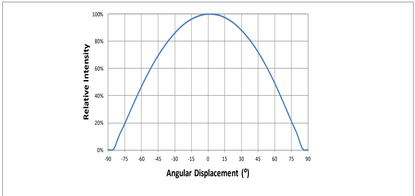
Figure 7: Typical Spatial Radiation Pattern at 20mA, T_{sp}=25^{\circ}\text{C}
