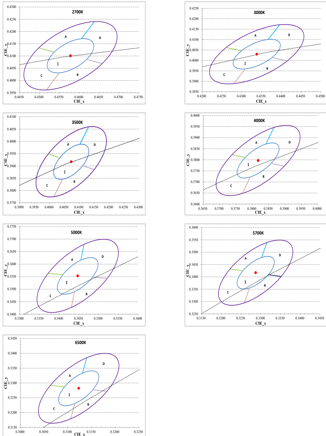
Figure 1: C.I.E. 1931 Chromaticity Diagram (Hot-color Targeted at T_{sp}=60^{\circ}\text{C}. )
