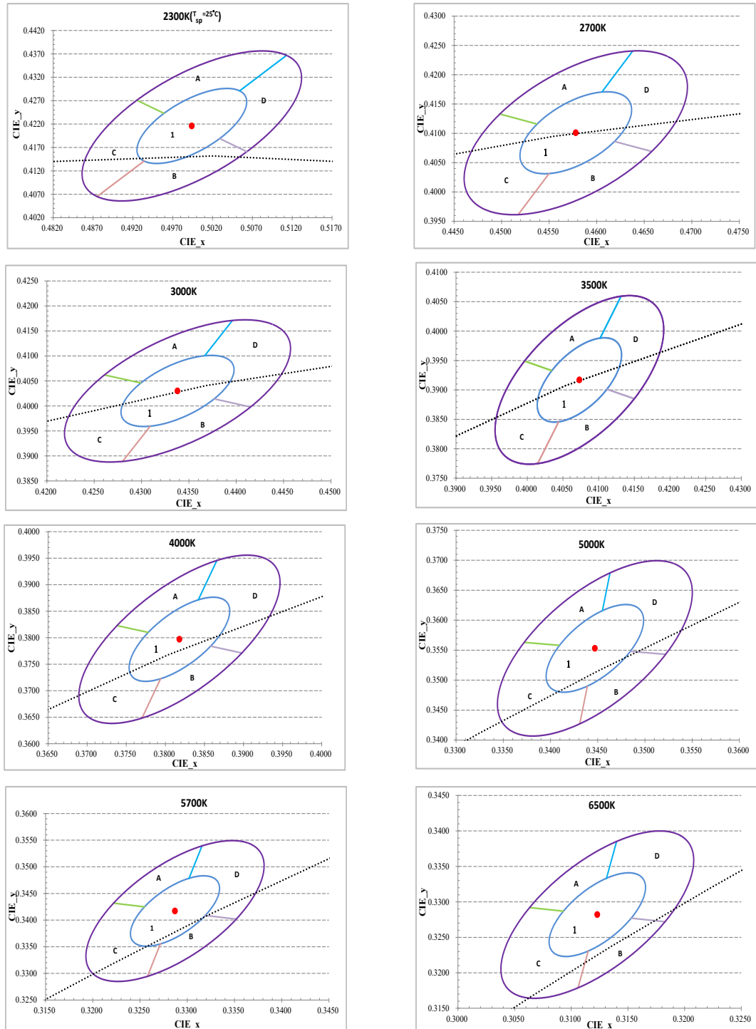
Figure 1: C.I.E. 1931 Chromaticity Diagram ( Hot-color Targeted at T_{sp}=60^{\circ}\text{C} , 2300K at T_{sp}=25^{\circ}\text{C} )
