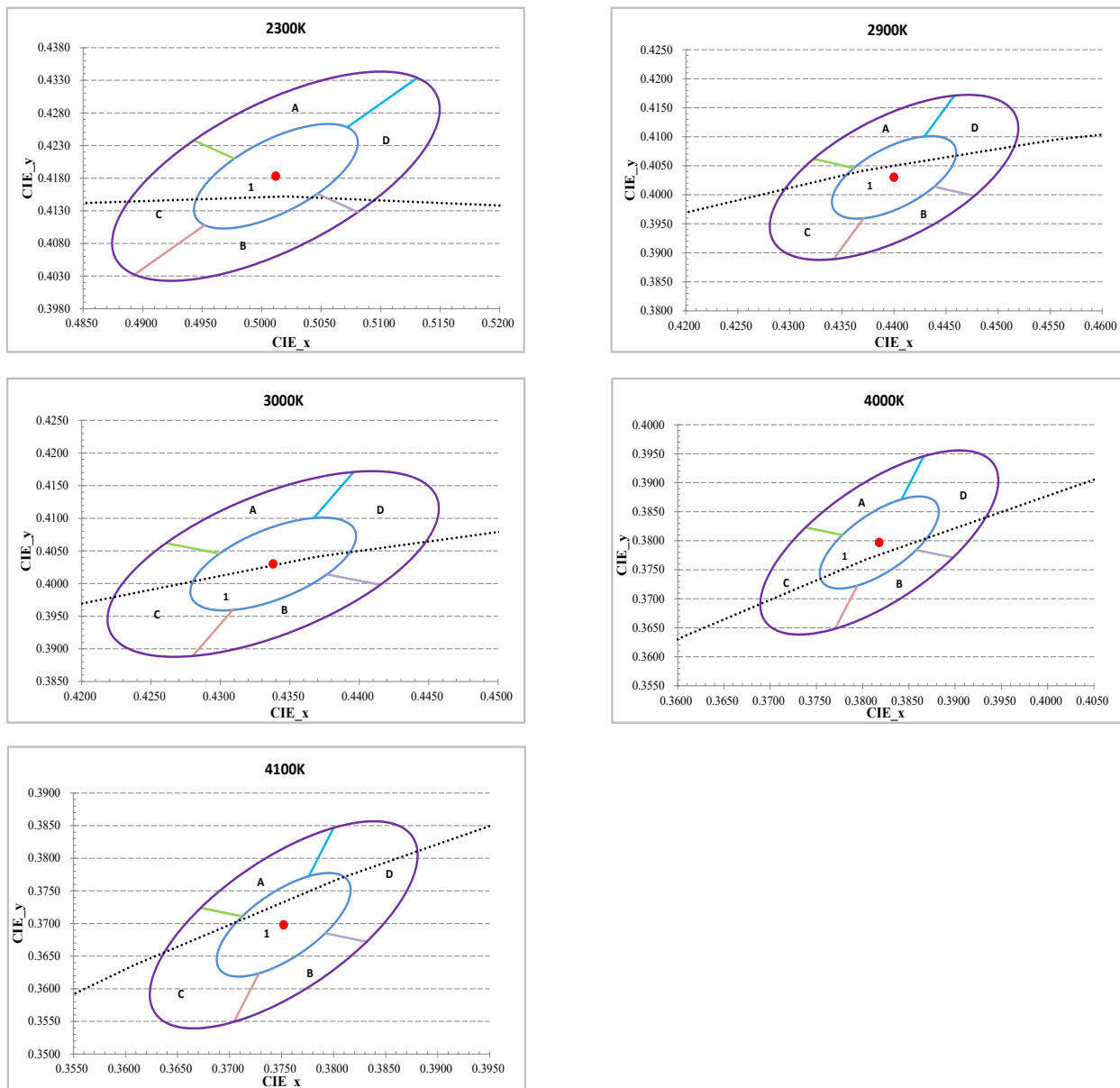
Figure 1: C.I.E. 1931 Chromaticity Diagram (5 Color Bin Structure, color Targeted at T_{sp} = 25^{\circ}\text{C} )
