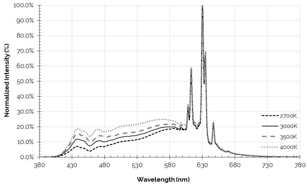
Figure 9: Typical Color Spectrum
