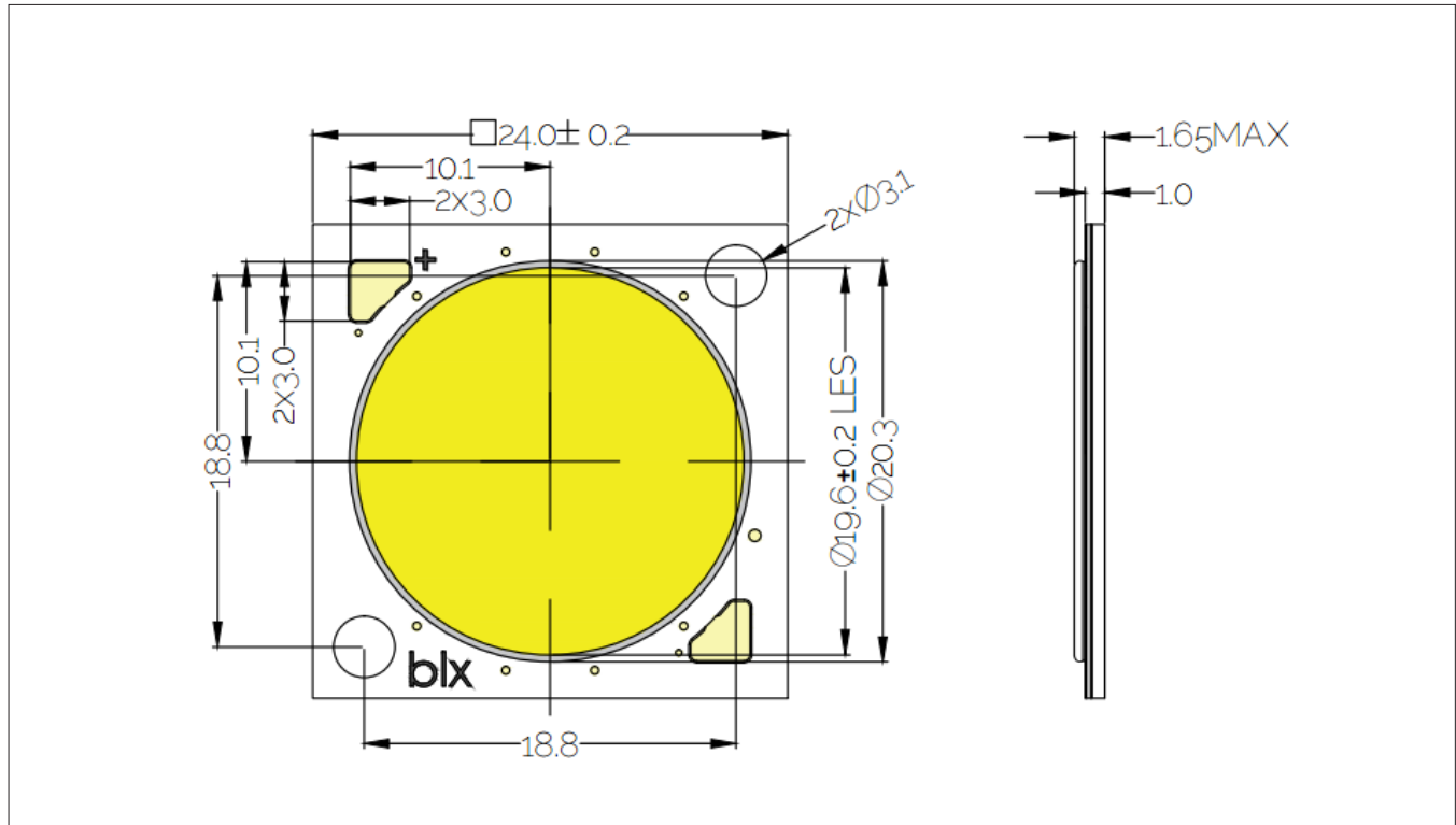
Figure 10: Drawing for V18 LED Array
