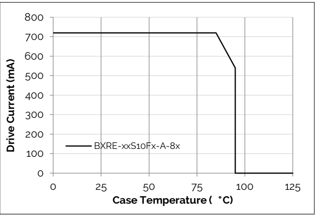
Figure 8: Derating Curve
