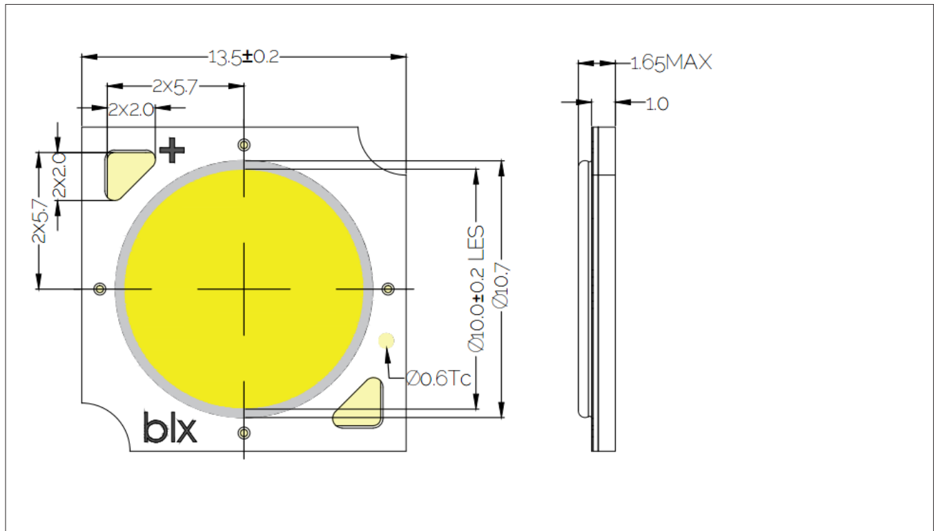
Figure 12: Drawing for V10 LED Array
