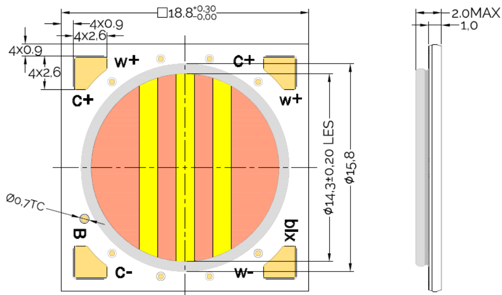
Figure 15: Drawing for Vesta Series Tunable White Gen 2 13mm Array
