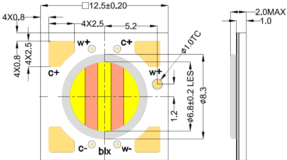
Figure 15: Drawing for Vesta Series Tunable White Gen2 6mm, 36V Array
