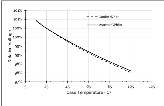
Figure 3: Relative Voltage vs. Case Temperature
