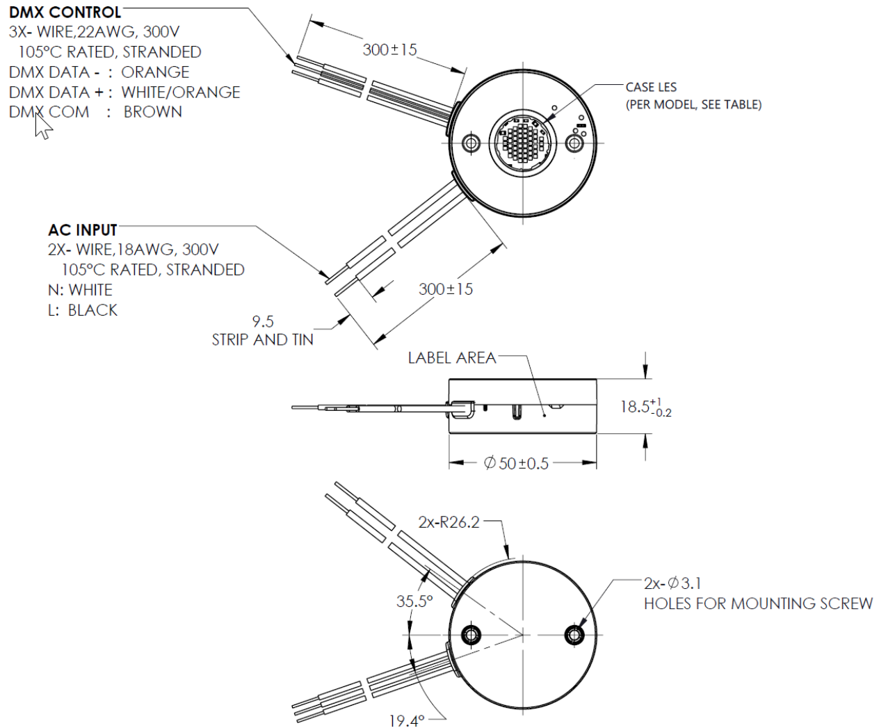
Figure 8: Mechanical Drawing (Side Cable Models)
