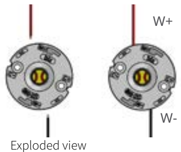
Electrical Connections
