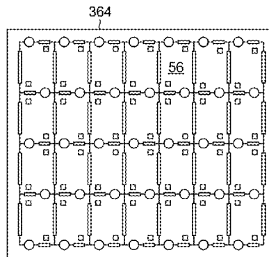
PANEL OF METAL CORE PRINTED CIRCUIT BOARDS
