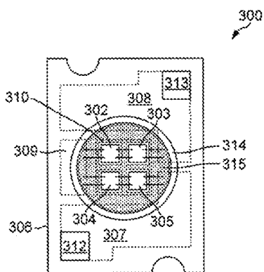
TOP-DOWN VIEW OF WHITE LED ASSEMBLY
