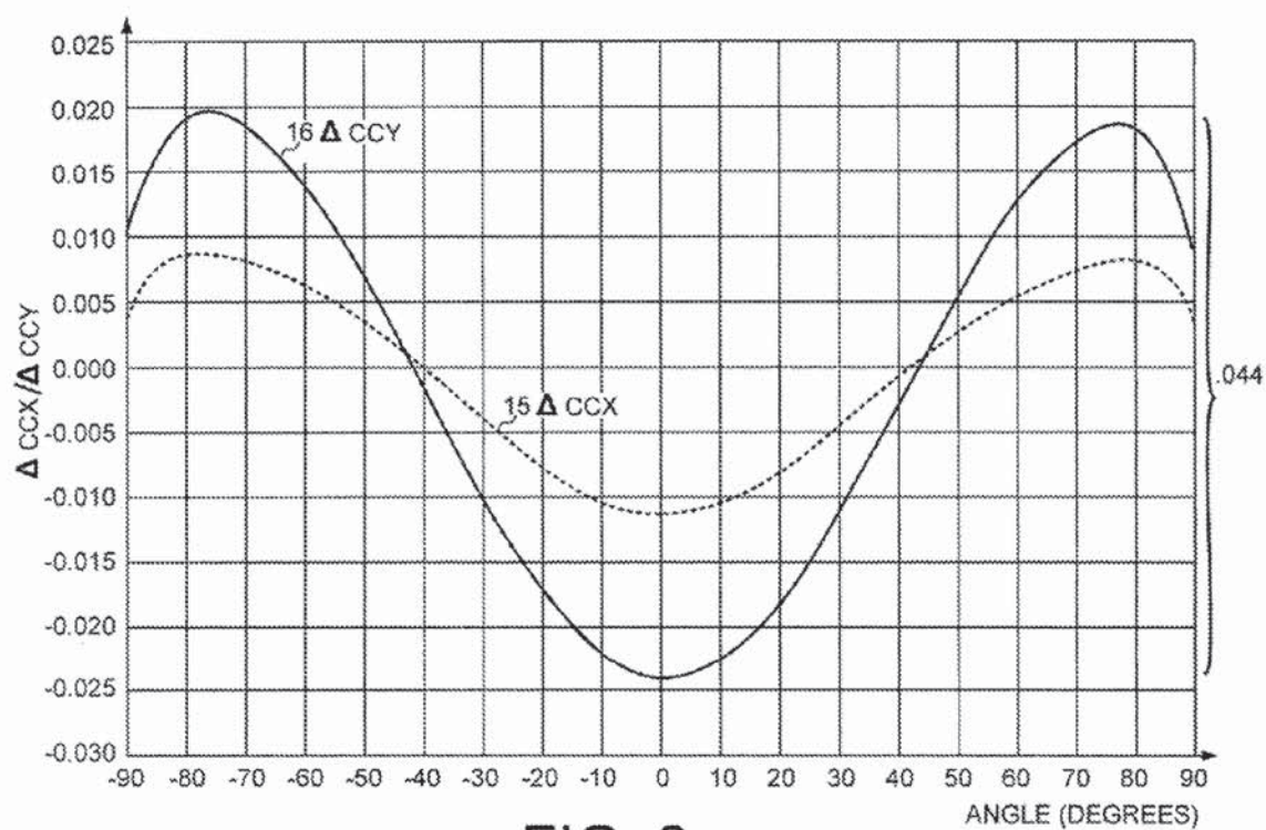
FIG. 2 (PRIOR ART)
