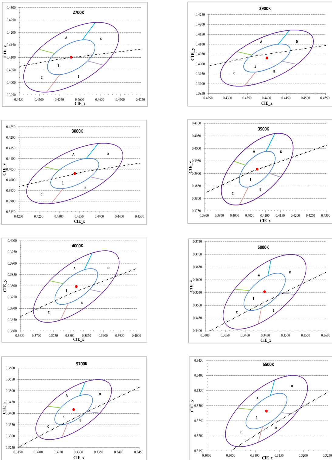
Figure 1: C.I.E. 1931 Chromaticity Diagram (5 Color Bin Structure, color Targeted at T_{sp} = 25^{\circ}\text{C} )
