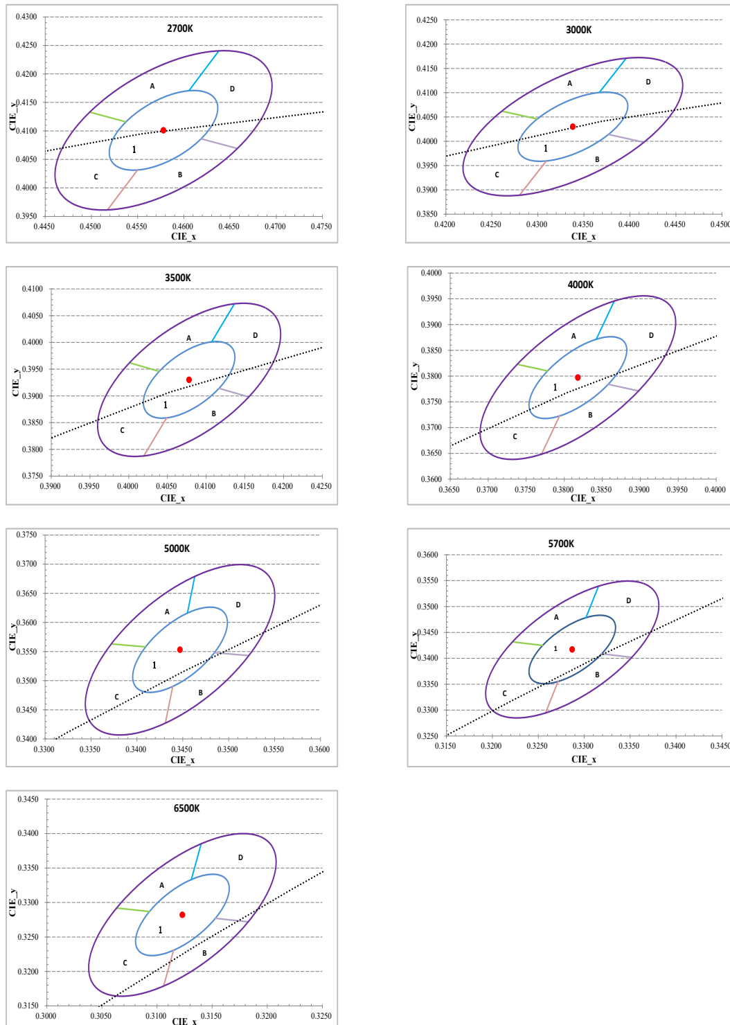
Figure 1: C.I.E. 1931 Chromaticity Diagram (5 Color Bin Structure, Hot-color Targeted at T_{sp} = 60^{\circ}\text{C} , )
