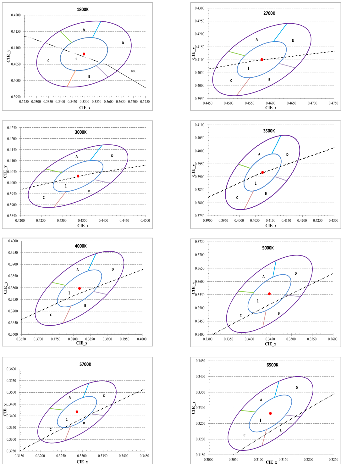
Figure 1: C.I.E. 1931 Chromaticity Diagram (5 Color Bin Structure, Cold-color Targeted at T_{sp}=25^{\circ}\text{C} )
