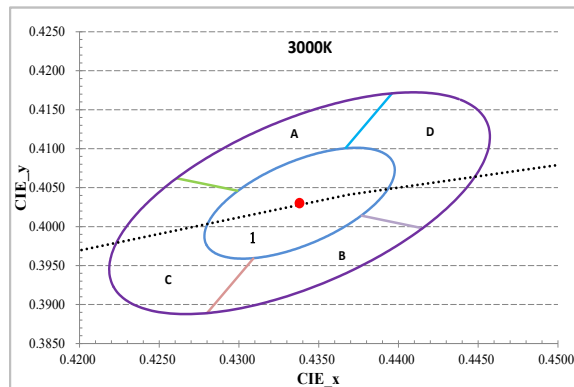
Figure 1: C.I.E. 1931 Chromaticity Diagram (5 Color Bin Structure, Cold-color Targeted at T_{sp} = 25^{\circ}\text{C} )
