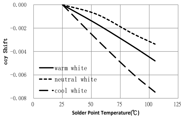
Figure 7: Typical c y Shift vs. Solder Point Temperature 2,3,4,5
