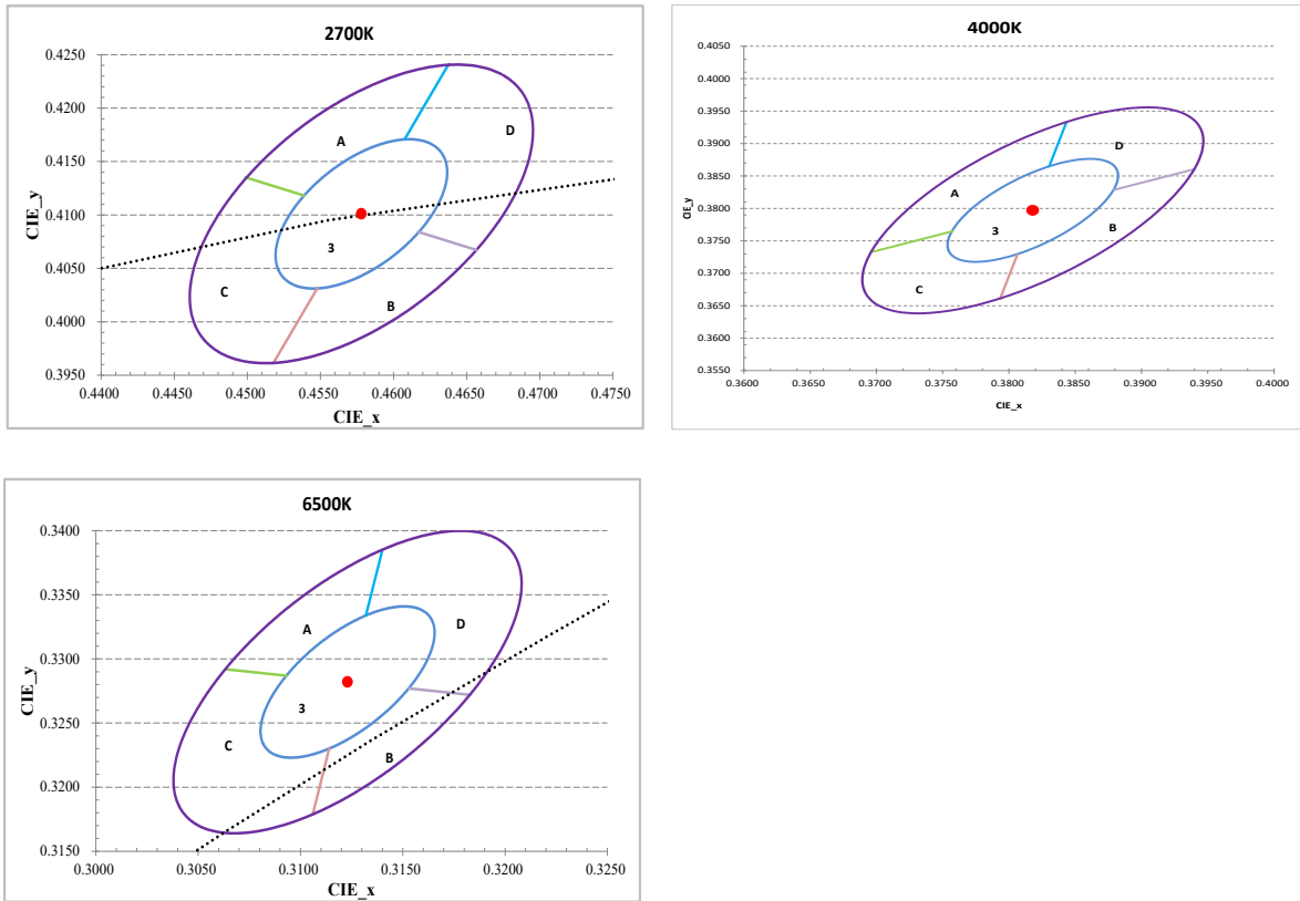
Figure 2: C.I.E. 1931 Chromaticity Diagram (Color Targeted at T_{sp}=55^{\circ}\text{C} )
