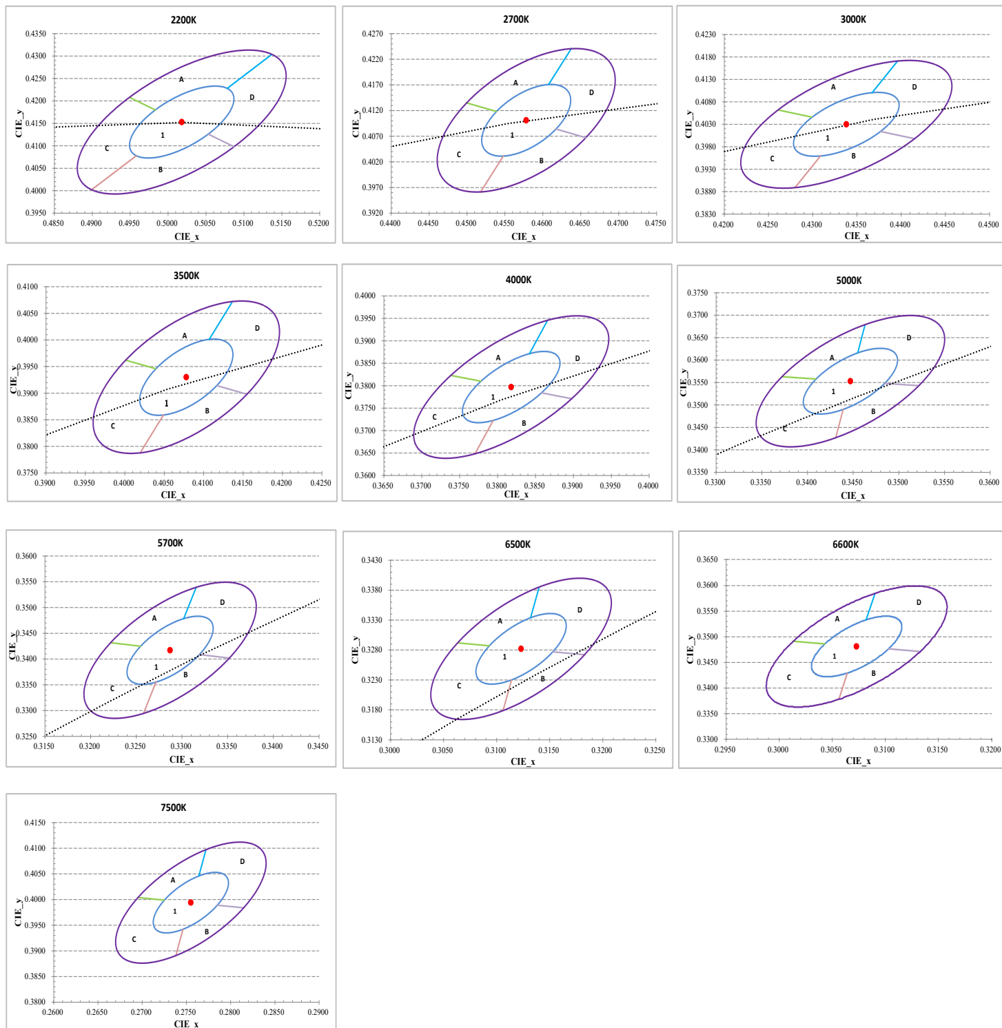
Figure 1: C.I.E. 1931 Chromaticity Diagram ( Cold-color Targeted at T_{sp}=25^{\circ}\text{C} )
