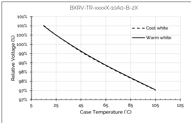
Figure 18: Relative Voltage vs. Case Temperature
