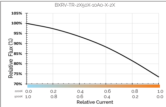
Figure 28: Relative Flux vs. Relative Current
