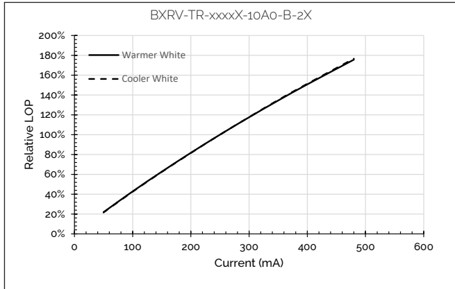
Figure 12: Relative Flux vs. Drive Current, T_c=25^\circ\text{C}
