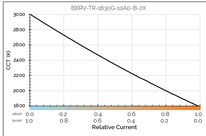
Figure 22: CCT vs. Relative Current, Tc=85°C
