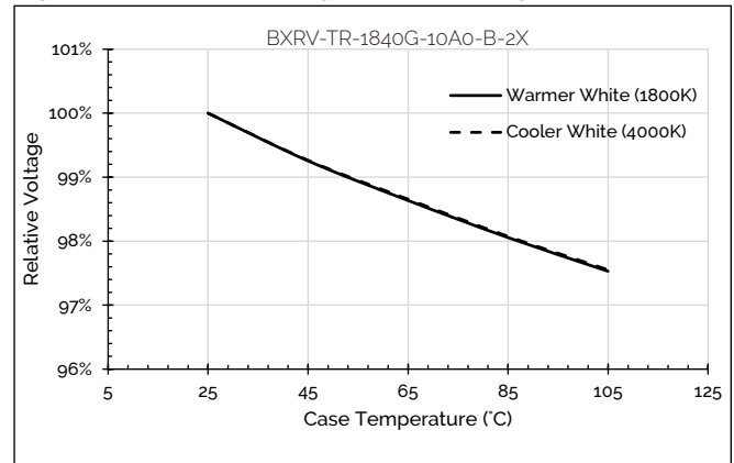
Figure 19: Relative Voltage vs. Case Temperature
