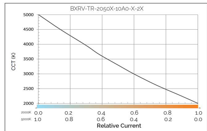
Figure 25: CCT vs. Relative Current, Tc=85°C
