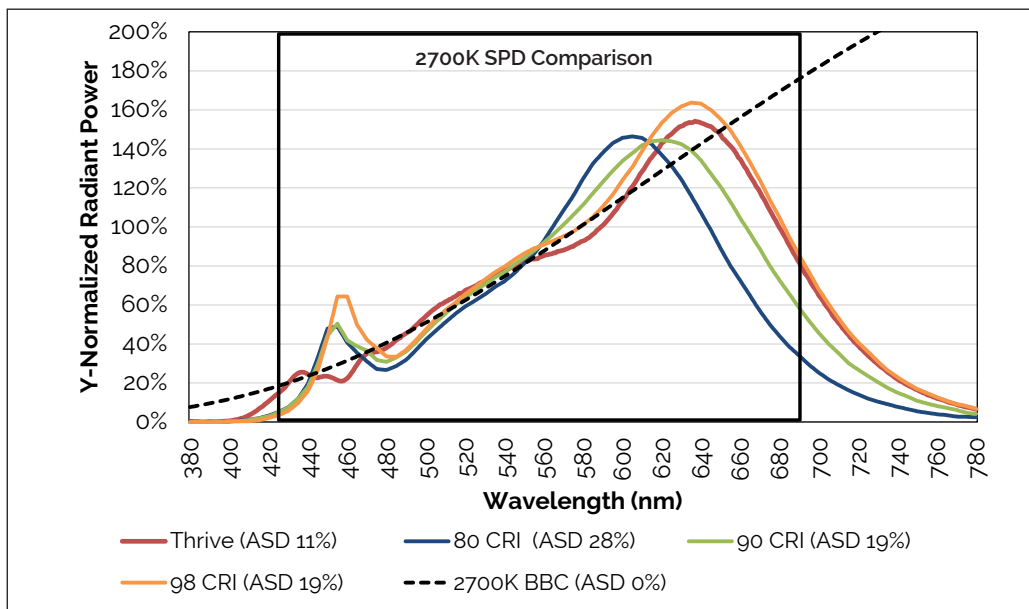
Figure 7: SPD Comparison
