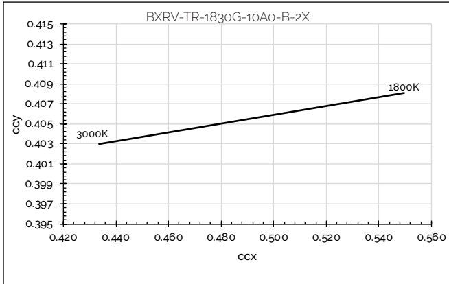
Figure 32: CCT Tuning Range, Tc=85°C
