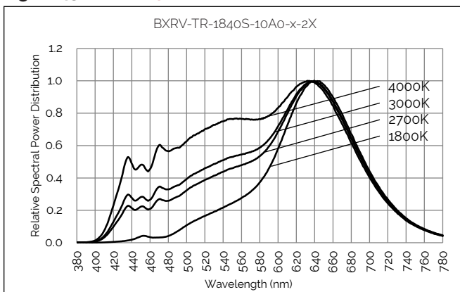
Figure 43: 1800K - 4000K with Thrive
