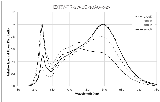
Figure 44: 2700K - 5000K with 90 CRI
