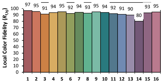
Figure 1: 2400K Thrive TM-30 Graphs
