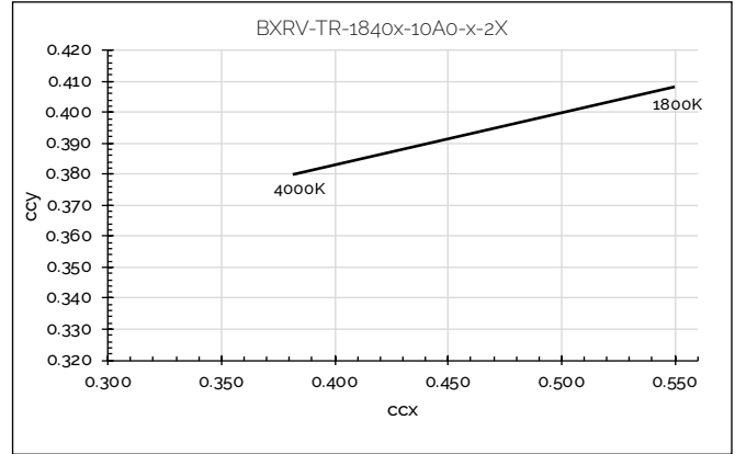
Figure 33: CCT Tuning Range, Tc=85°C
