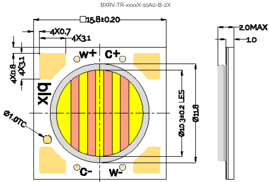
Figure 49: Drawing for Vesta Series Tunable White Gen2 9mm, 36V Array
