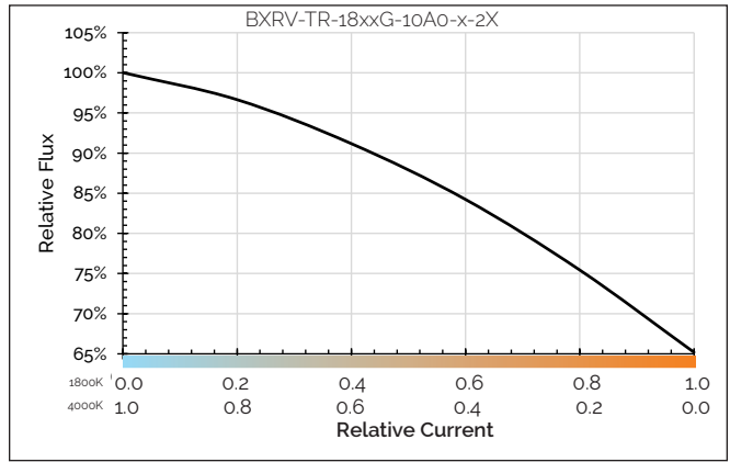
Figure 29: Relative Flux vs. Relative Current
