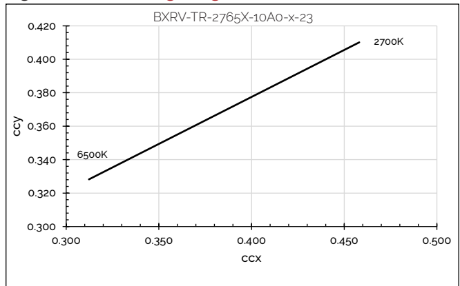
Figure 31: CCT Tuning Range, Tc=85°C
