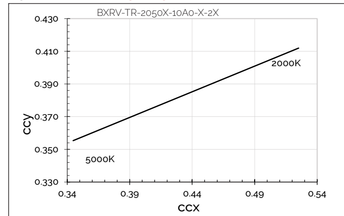
Figure 35: CCT Tuning Range, Tc=85°C
