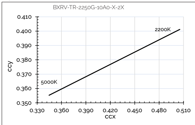
Figure 34: CCT Tuning Range, Tc=85°C
