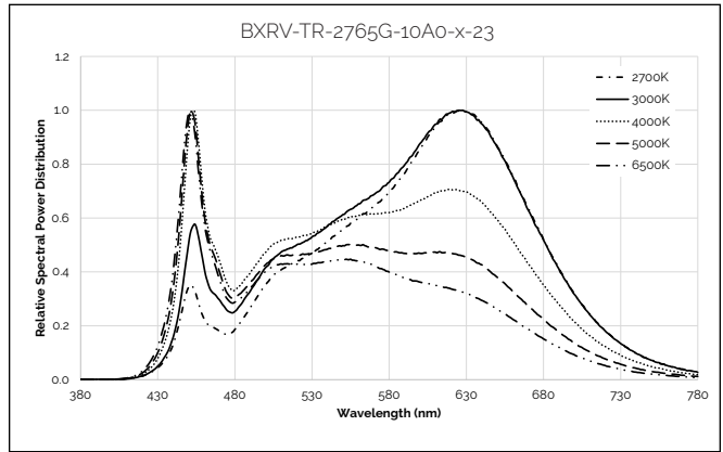
Figure 45: 2700K - 6500K with 90 CRI
