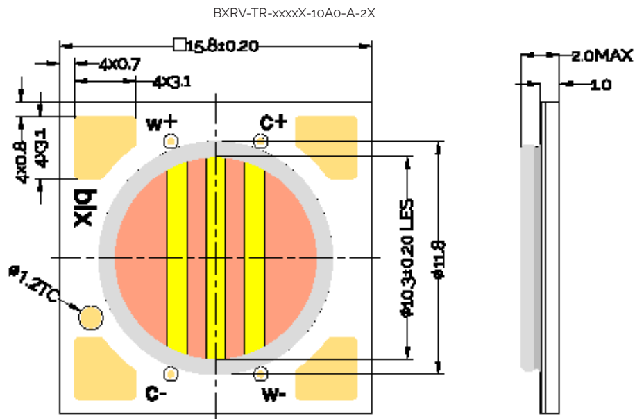
Figure 50: Drawing for Vesta Series Tunable White Gen2 9mm, 18V Array
