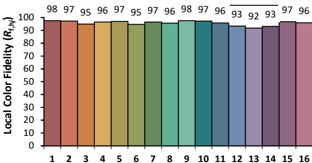
Figure 1: 2400K Thrive TM-30 Graphs
