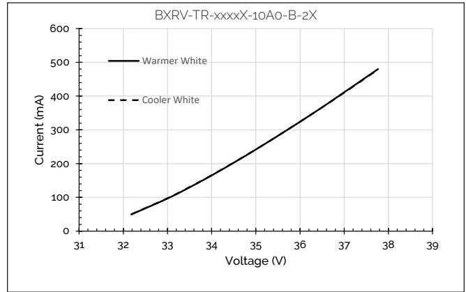
Figure 9: Forward Voltage vs. Forward Current, T_c=25^\circ\text{C}
