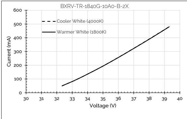
Figure 10: Forward Voltage vs. Forward Current, T_c=25^\circ\text{C}
