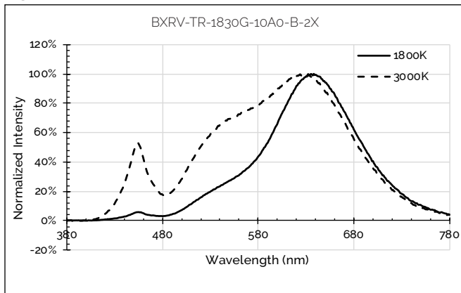
Figure 46: 1800K - 3000K with 90 CRI
