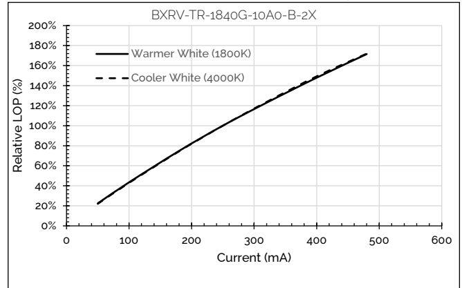
Figure 13: Relative Flux vs. Drive Current, T_c=25^\circ\text{C}
