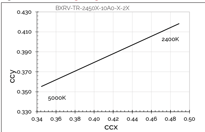
Figure 36: CCT Tuning Range, Tc=85°C
