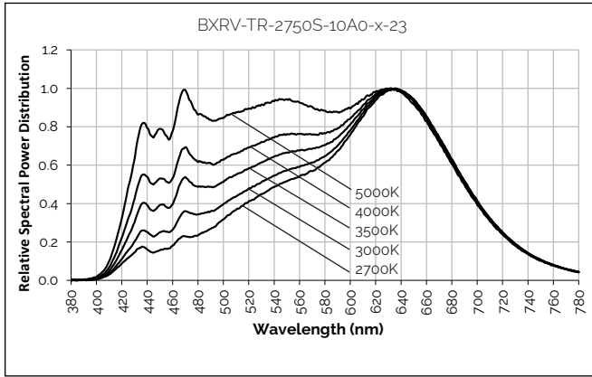
Figure 39: 2700K - 5000K with Thrive
