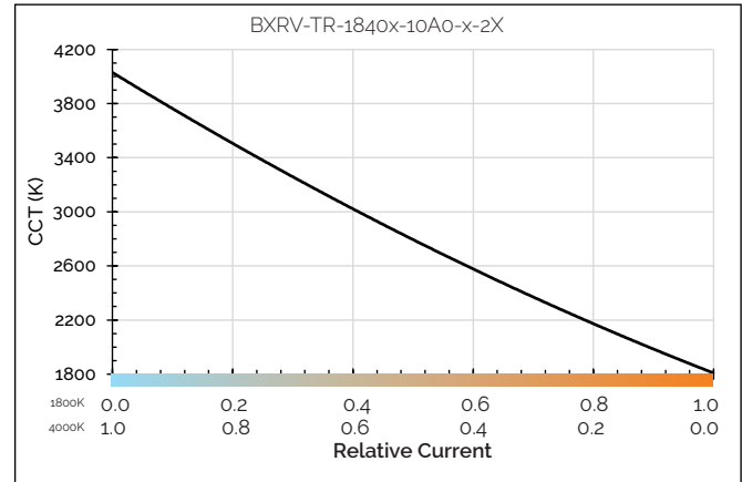
Figure 23: CCT vs. Relative Current, Tc=85°C
