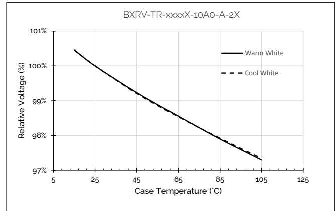
Figure 17: Relative Voltage vs. Case Temperature
