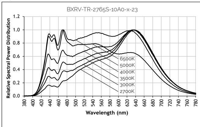
Figure 41: 2700K - 6500K with Thrive
