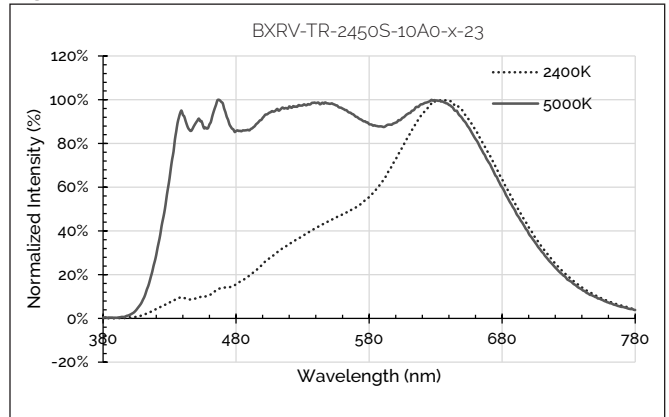
Figure 42: 2400K - 5000K with Thrive
