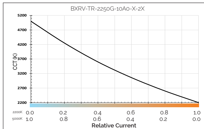
Figure 24: CCT vs. Relative Current, Tc=85°C
