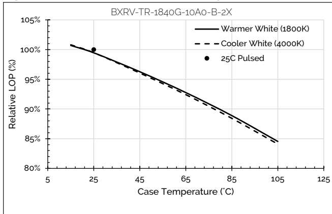
Figure 16: Relative Flux vs. Case Temperature
