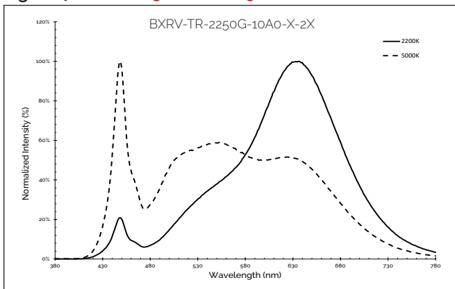
Figure 48: 2200K - 5000K with 90 CRI
