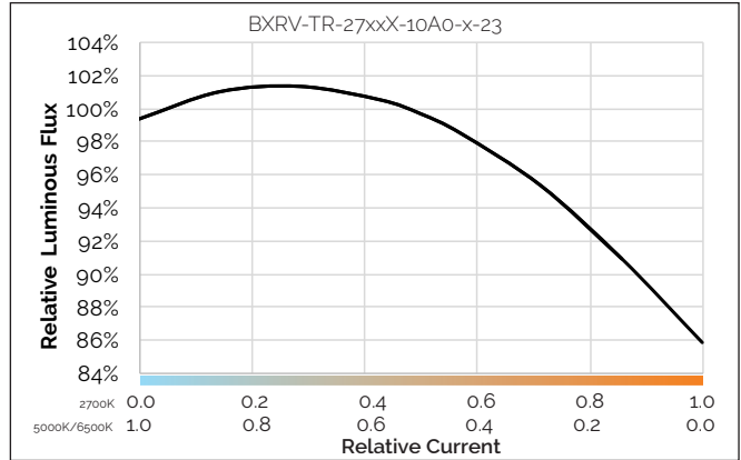
Figure 27: Relative Flux vs. Relative Current
