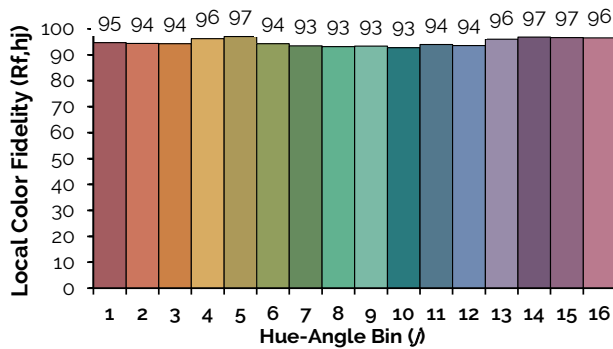
Figure 5: 5000K Thrive TM-30 Graphs
