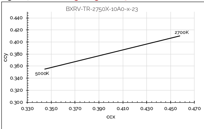
Figure 30: CCT Tuning Range, Tc=85°C
