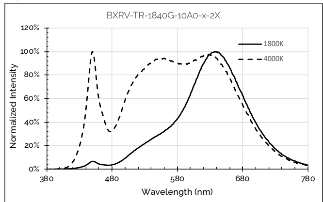
Figure 47: 1800K - 4000K with 90 CRI
