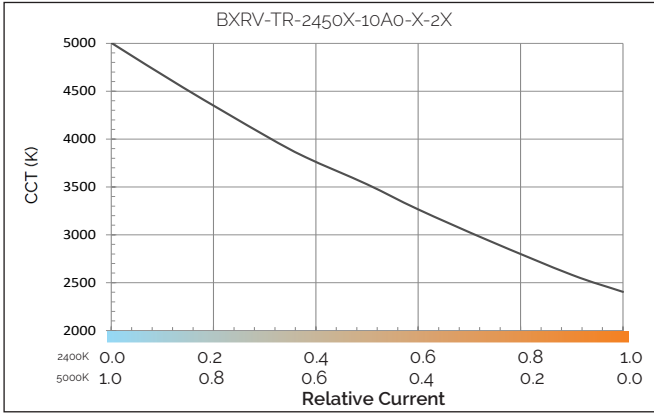
Figure 26: CCT vs. Relative Current, Tc=85°C
