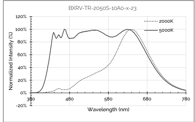
Figure 40: 2000K - 5000K with Thrive
