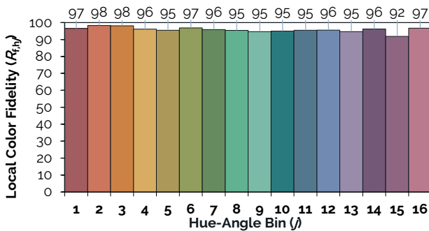
Figure 6: 6500K Thrive TM-30 Graphs
