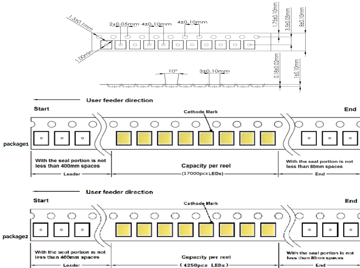
Figure 19: Emitter Tape Drawings
