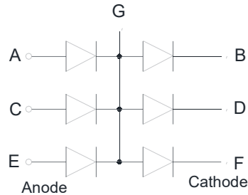
Equivalent Circuit
