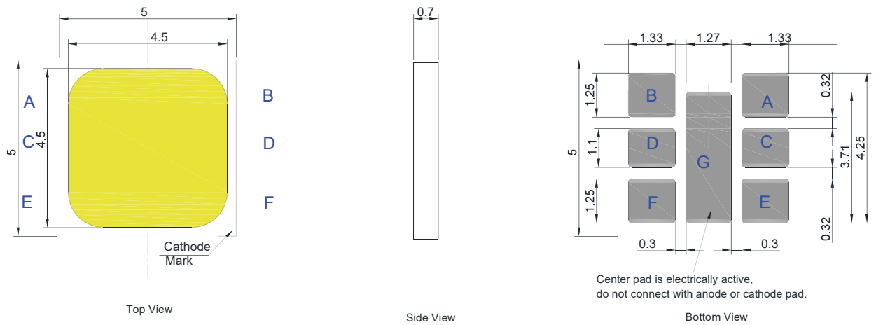
Figure 11: Drawing for SMD 5050
