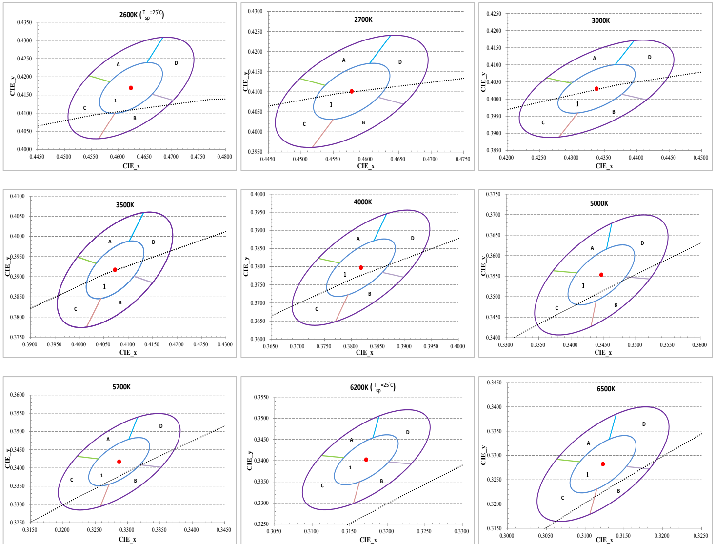
Figure 1: C.I.E. 1931 Chromaticity Diagram (5 Color Bin Structure, Hot-color Targeted at T_{sp}=85^{\circ}\text{C} , 2600K/6200K at T_{sp}=25^{\circ}\text{C} )
