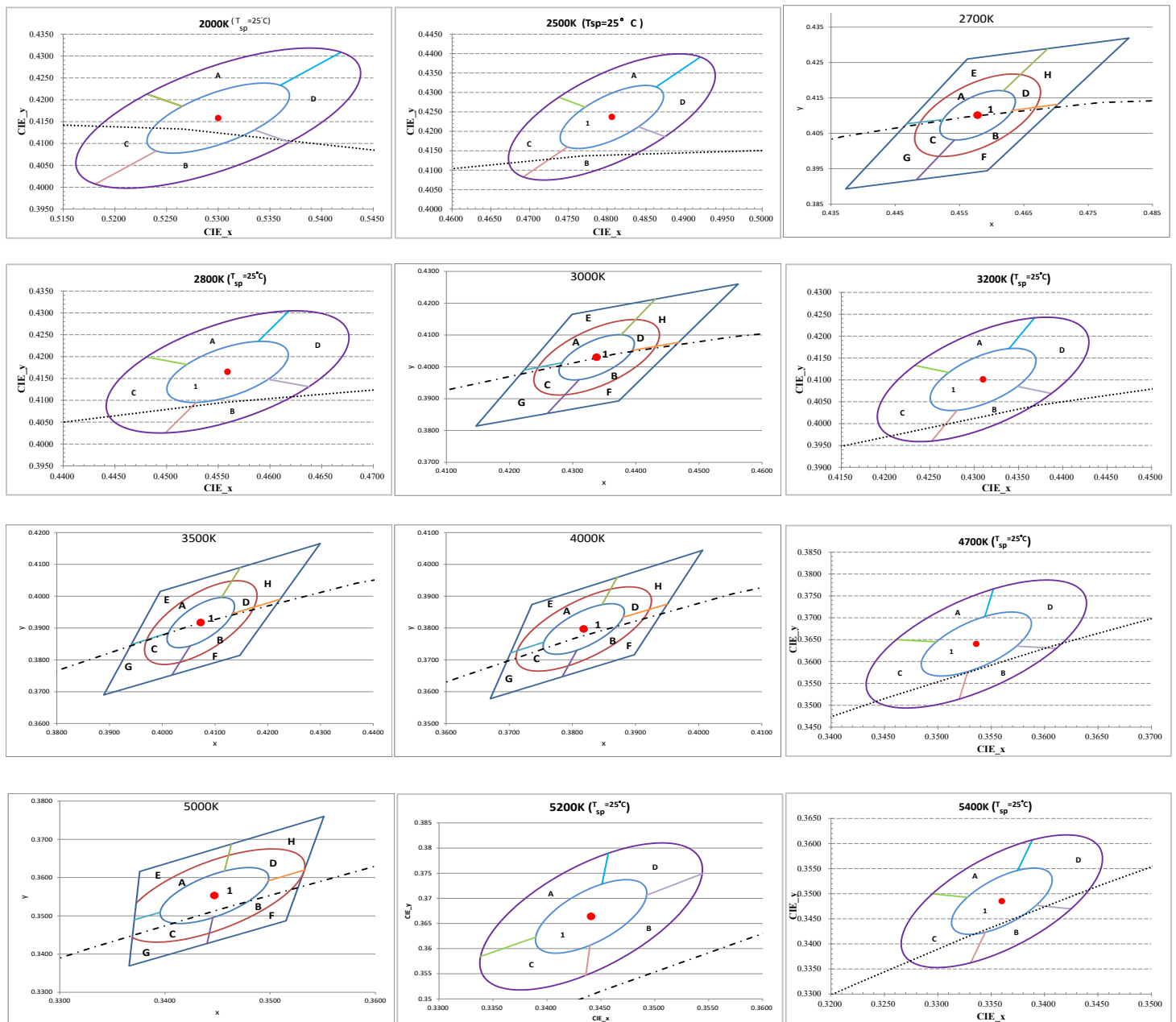
Figure 1: C.I.E. 1931 Chromaticity Diagram (Hot-color Targeted at T_{sp}=85^{\circ}\text{C} . 2000K/2500K/2800K/3200K/4700K/5200K/5400K/5900K/6200K/7100K= T_{sp}=25^{\circ}\text{C} .)
