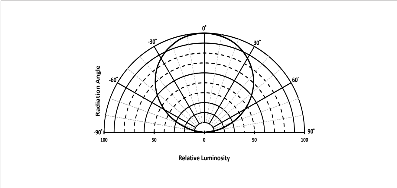
Figure 8: Typical Polar Radiation Pattern at 25mA, T sp = 25°C
