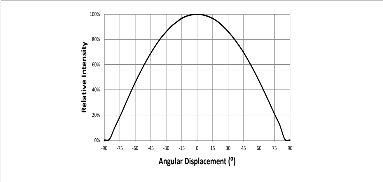
Figure 7: Typical Spatial Radiation Pattern at 25mA, T sp = 25°C
