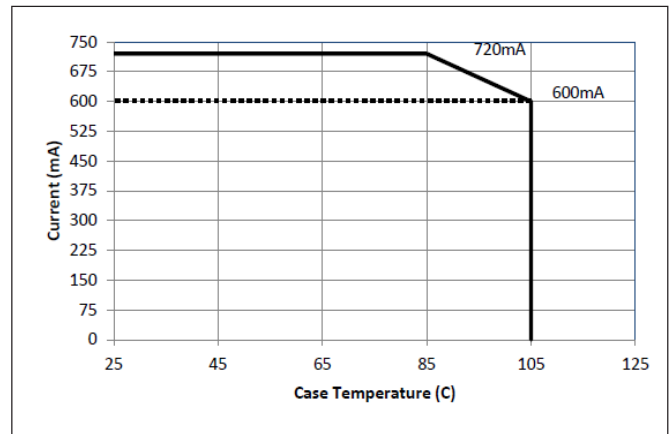
Figure 8: Derating Curve
