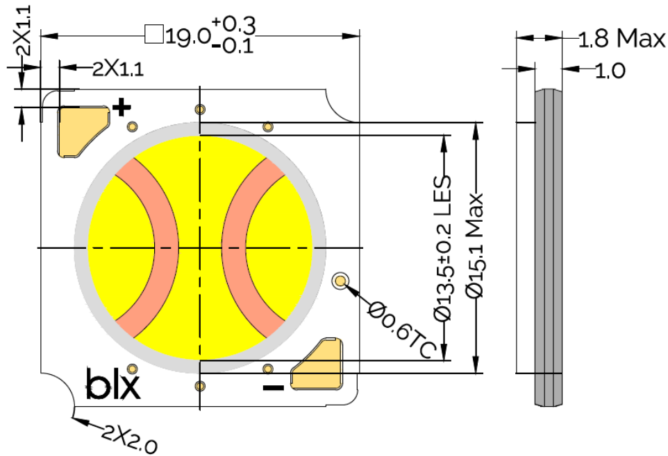
Figure 12: Mechanical Drawing Specifications
