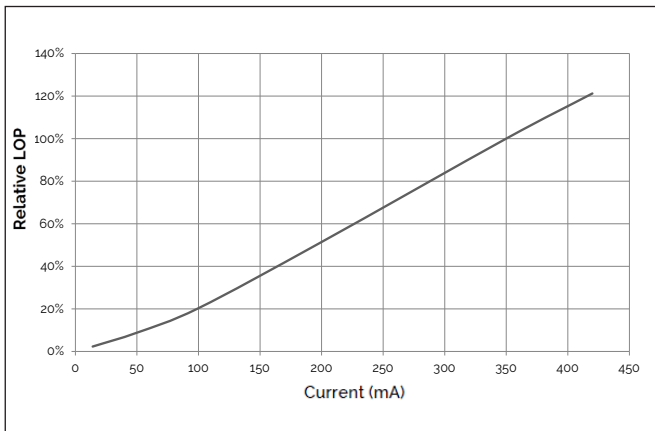
Figure 3: Relative LOP vs. Drive Current, T_c=25^\circ\text{C}
