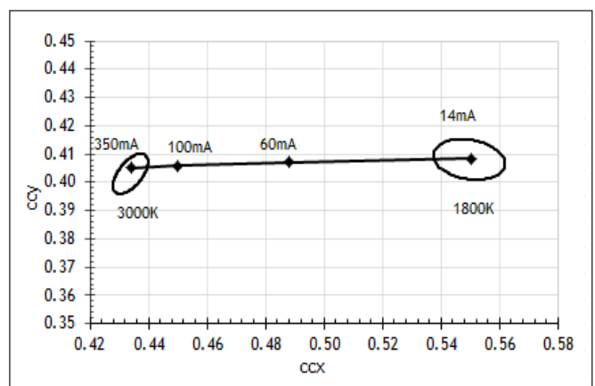
Figure 6: Color shift vs. Forward Current 3000K - 1800K
