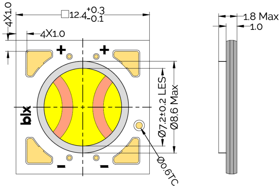
Figure 12: Mechanical Drawing Specifications
