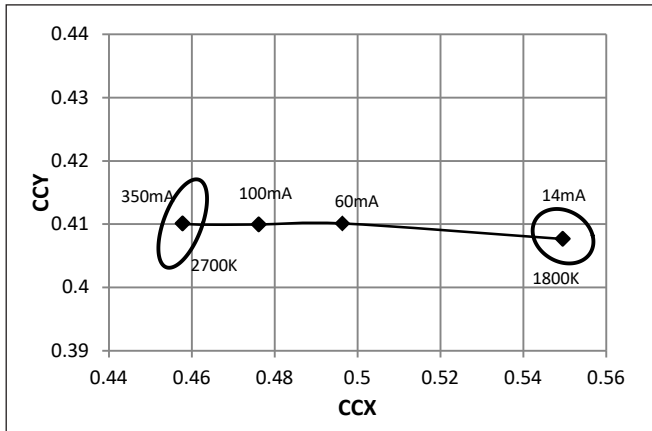
Figure 7: Color shift vs. Forward Current 2700K - 1800K
