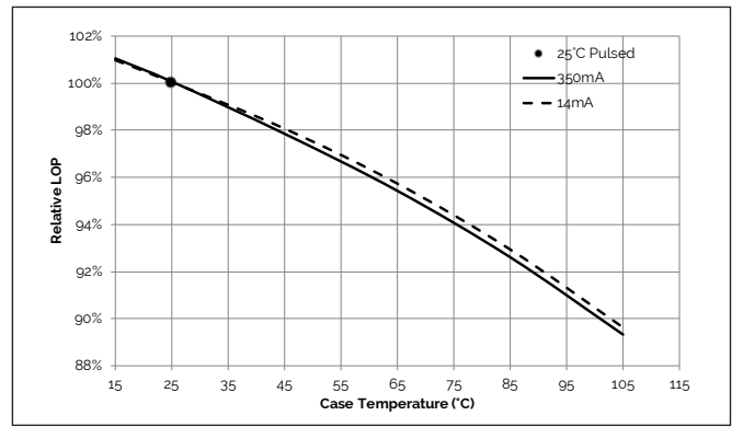
Figure 2: Relative Flux vs. Case Temperature
