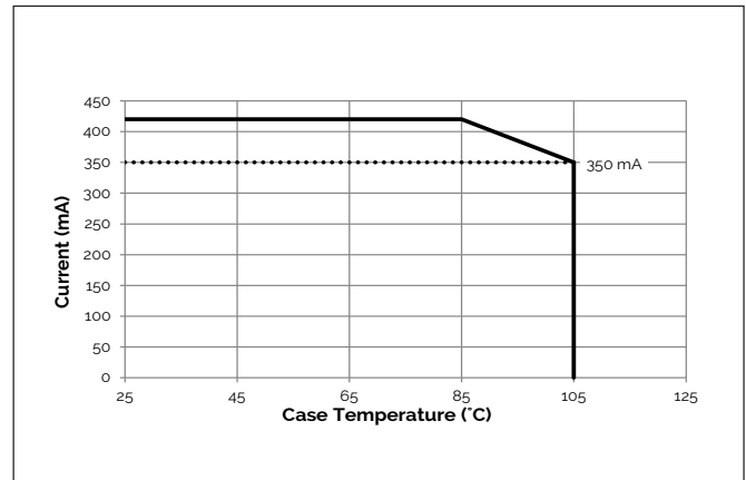
Figure 8: Derating Curve
