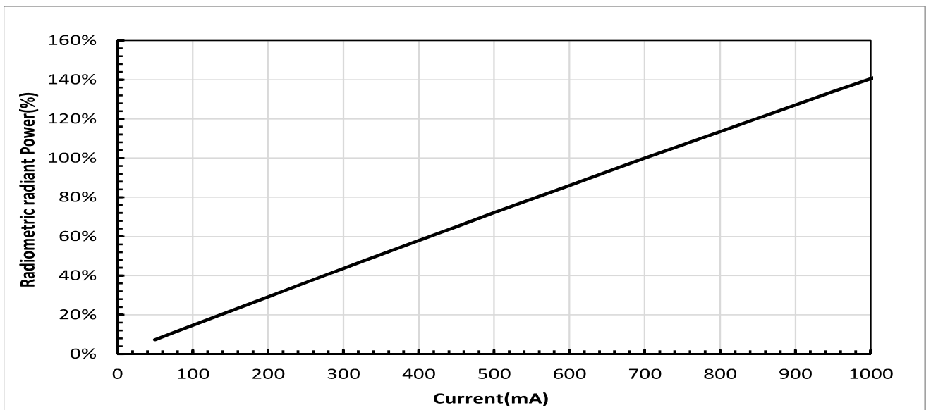
Figure 2: Relative Total Radiant Radiometric vs. Drive Current ( T_{sp}=25^{\circ}\text{C} )
