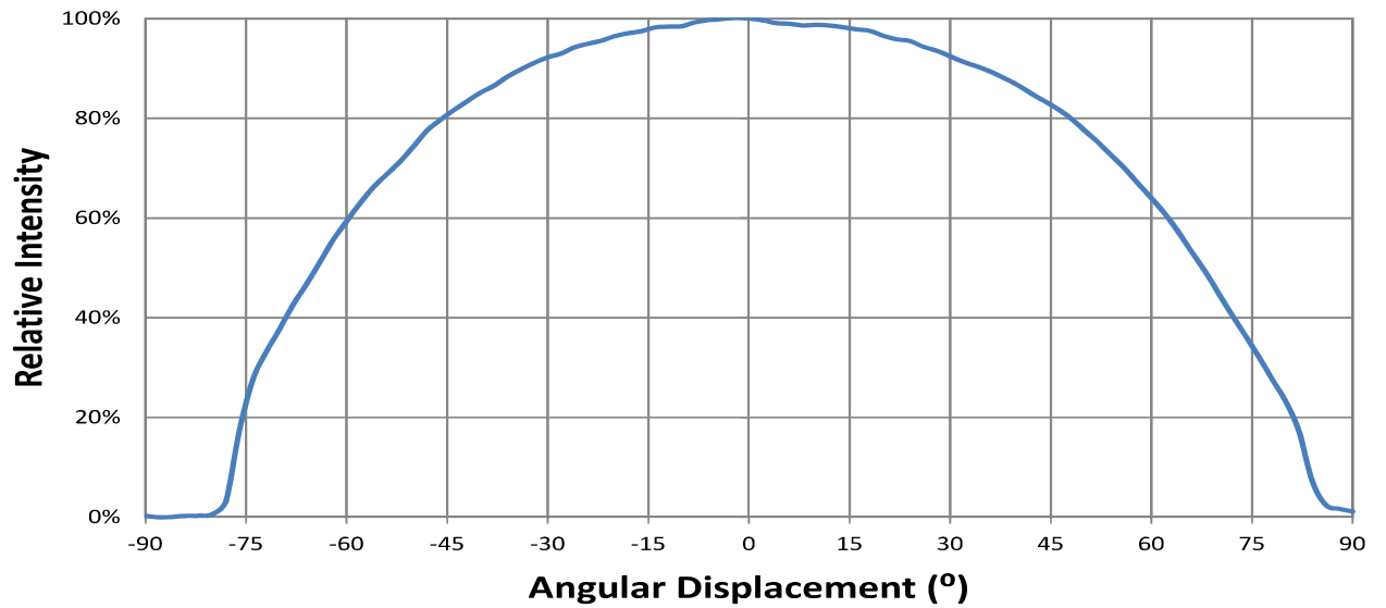
Figure 5: Typical Spatial Radiation Pattern at 700mA, T_{sp}=25^{\circ}\text{C}
