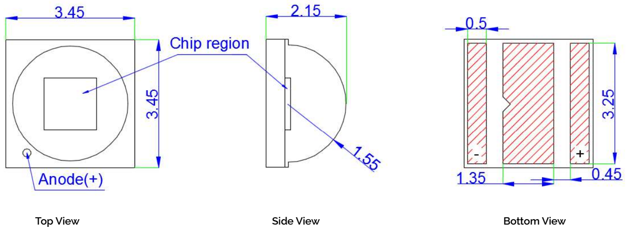
Figure 8: Drawing for SMD 3535
