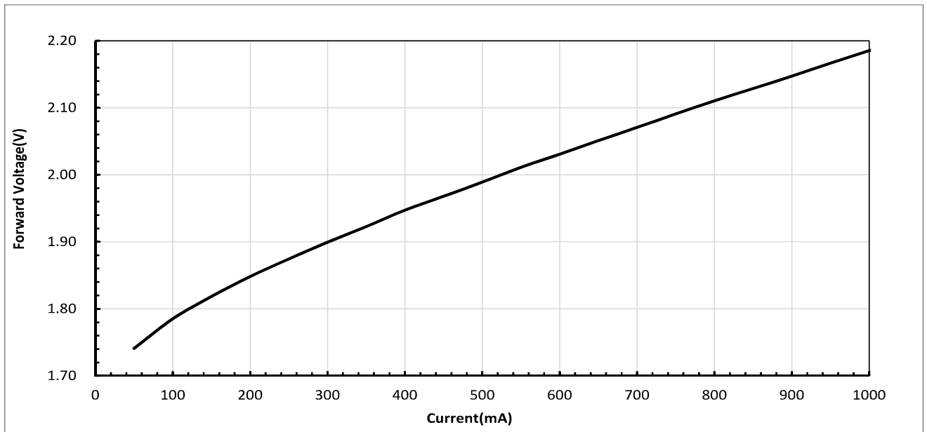
Figure 1: Drive Current vs. Relative Voltage ( T_{sp}=25^{\circ}\text{C} )
