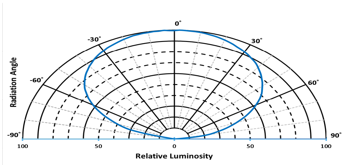
Figure 6: Typical Polar Radiation Pattern at 700mA, T_{sp}=25^{\circ}\text{C}
