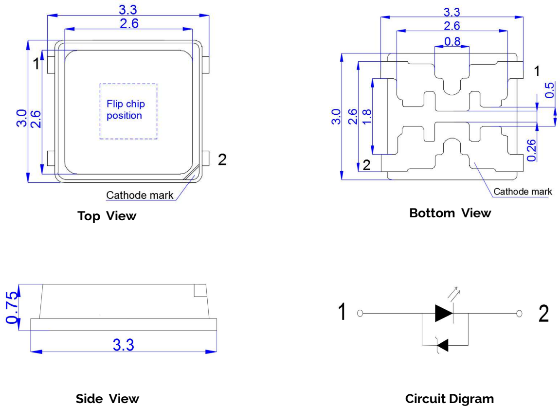
Figure 11: Drawing for SMD 3030
