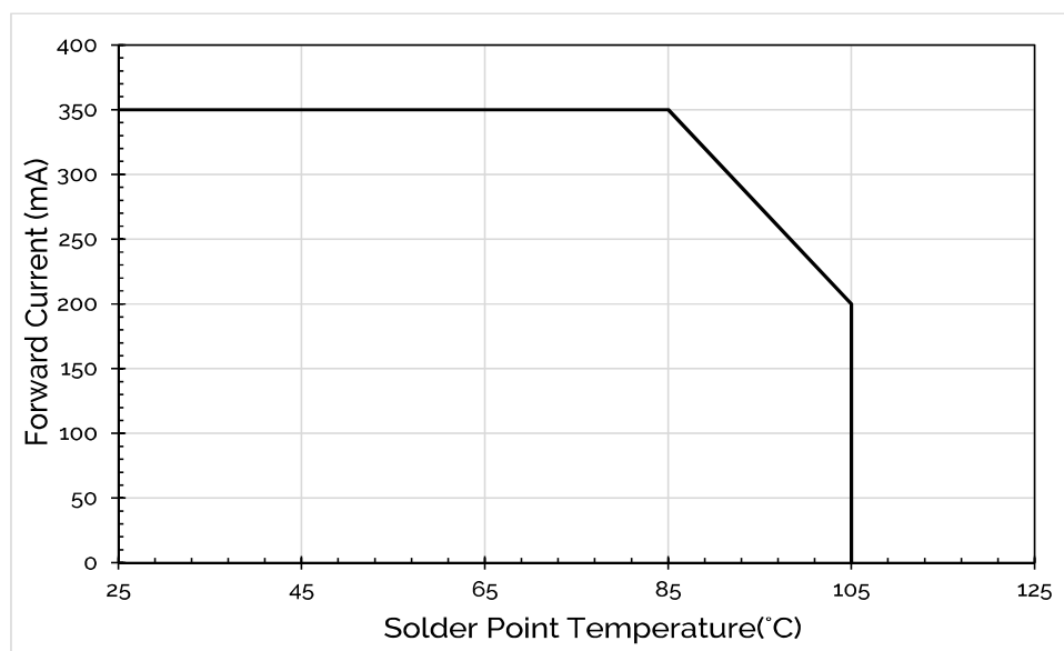
Figure 7: Drive Current vs Solder Point Temperature
