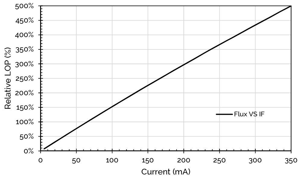
Figure 3: Typical Relative Luminous Flux vs. Forward Current ( T_{sp}=25^{\circ}\text{C} )
