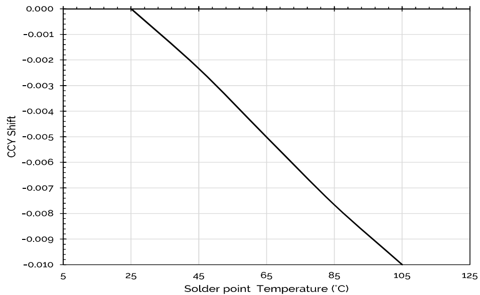
Figure 6: Typical ccy Shift vs. Solder Point Temperature
