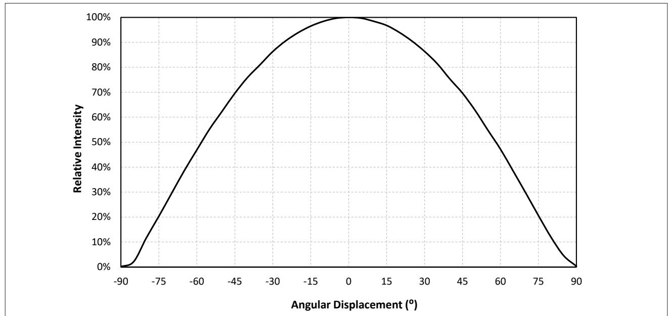
Figure 7: Typical Spatial Radiation Pattern at 160mA, T_{sp}=25^{\circ}\text{C}
