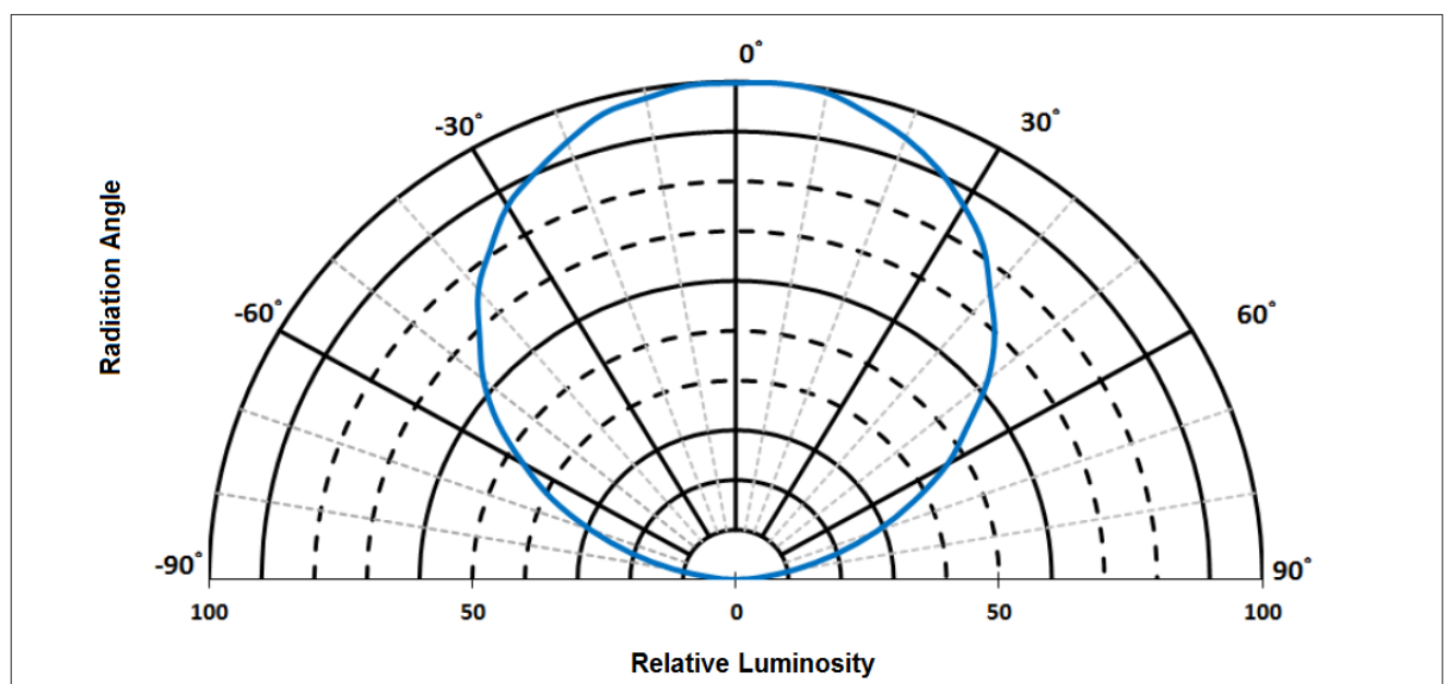
Figure 8: Typical Polar Radiation Pattern at 160mA, T_{sp}=25^{\circ}\text{C}
