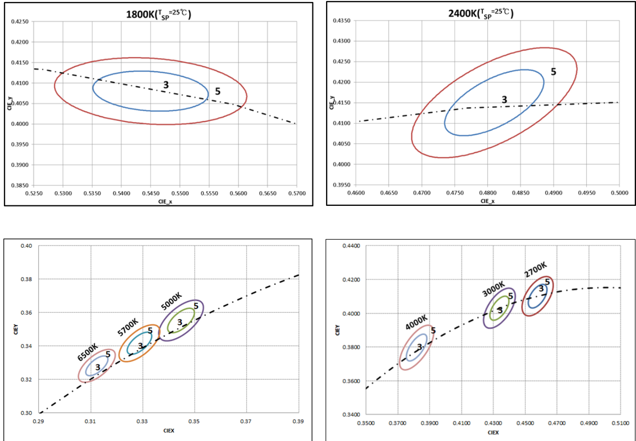
Figure 1: C.I.E. 1931 Chromaticity Diagram (2 Color Bin Structure, Hot-color Targeted at T_{sp}=85^{\circ}\text{C} )
