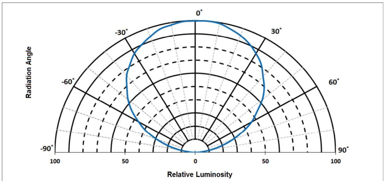
Figure 9: Typical Polar Radiation Pattern at 0mA, T_{sp}=25^{\circ}\text{C}
