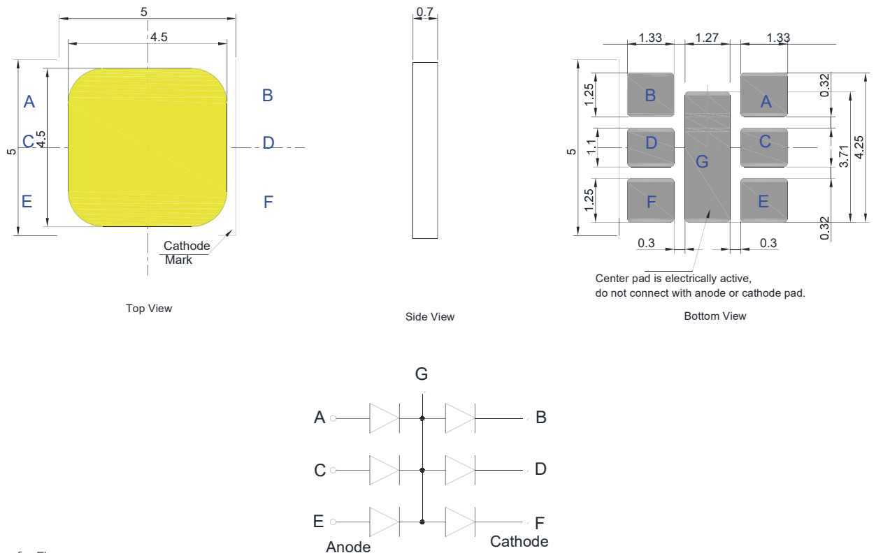
Equivalent Circuit
