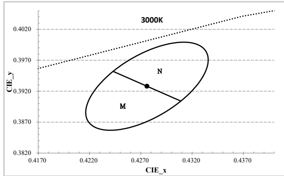
Figure 1: C.I.E. 1931 Chromaticity Diagram (2 Color Bin Structure, Cold-color Targeted at T_{sp}=25^{\circ}\text{C} )
