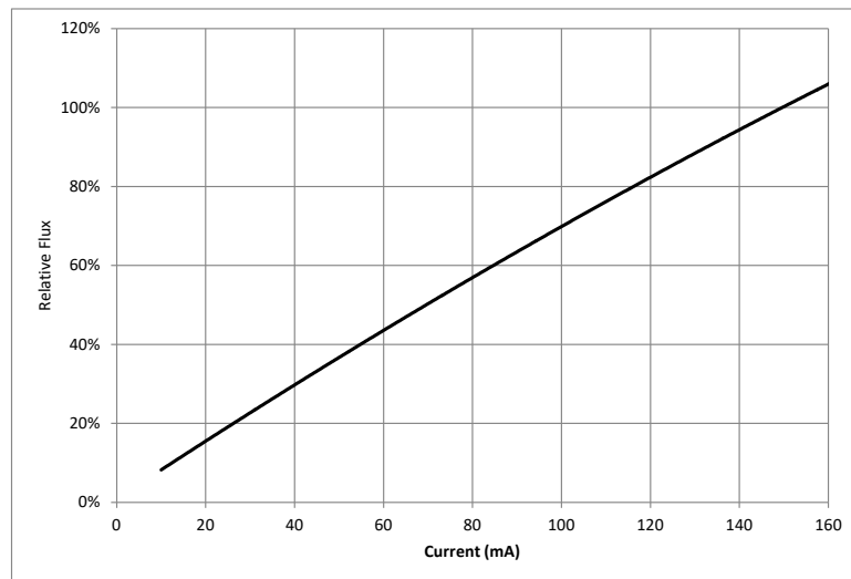
Figure 3: Typical Relative Luminous Flux vs. Forward Current ( T_{sp}=25^{\circ}\text{C} )
