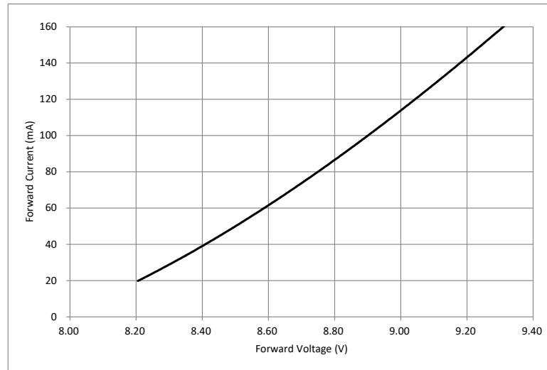
Figure 2: Drive Current vs. Voltage ( T_{sp}=25^{\circ}\text{C} )
