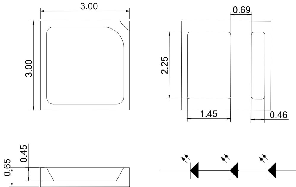
Figure 10: Drawing for SMD 3030
