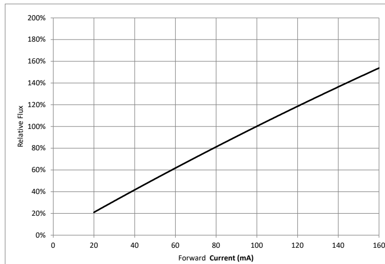
Figure 3: Typical Relative Luminous Flux vs. Drive Current ( T_{sp}=25^{\circ}\text{C} )
