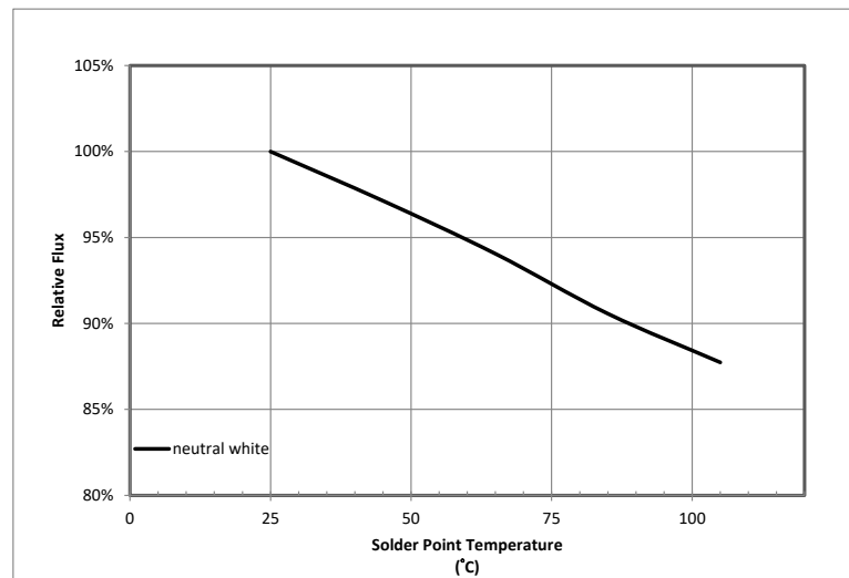
Figure 4: Typical Relative Flux vs. Solder Point Temperature
