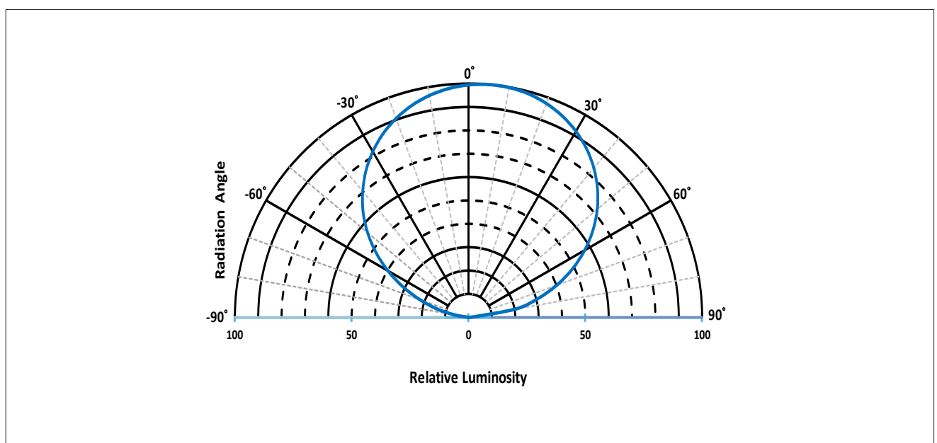
Figure 8: Typical Polar Radiation Pattern at 42mA, T_{sp}=25^{\circ}\text{C}
