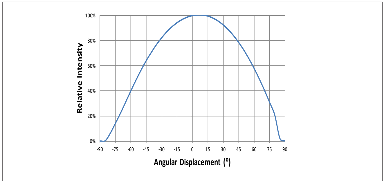
Figure 7: Typical Spatial Radiation Pattern at 42mA, T_{sp}=25^{\circ}\text{C}
