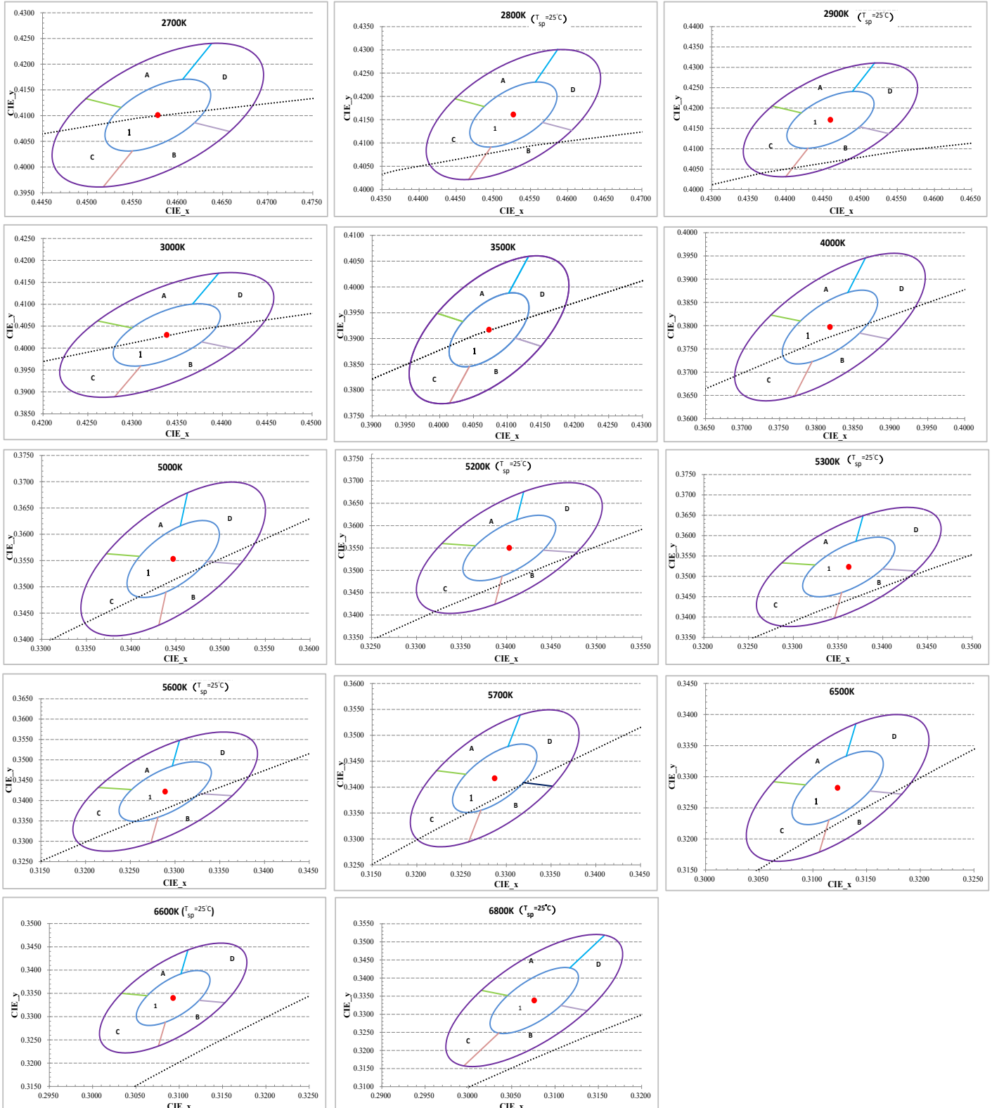
Figure 1: C.I.E. 1931 Chromaticity Diagram ( 5 Color Bin Structure, color Targeted at T_{sp}=85^{\circ}\text{C} ,
