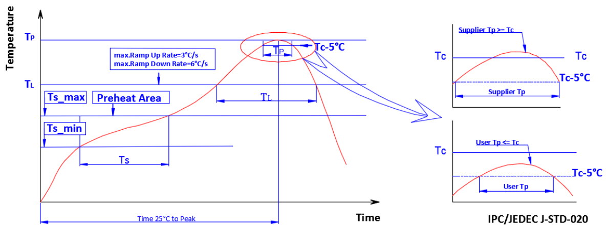
Figure 12 : Reflow Profile
