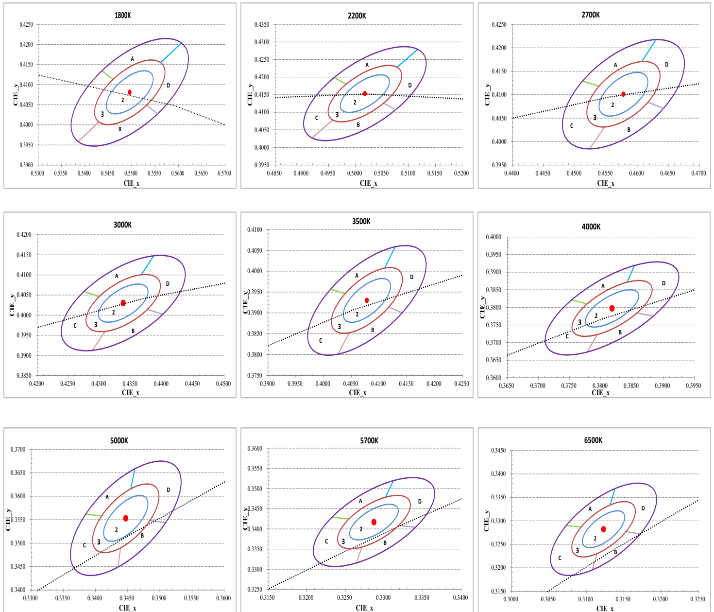
Figure 1: C.I.E. 1931 Chromaticity Diagram ( Cold-color Targeted at T_{sp}=25^{\circ}\text{C} )
