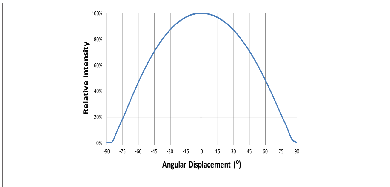
Figure 7: Typical Spatial Radiation Pattern at 300mA, T_{sp}=25^{\circ}\text{C}
