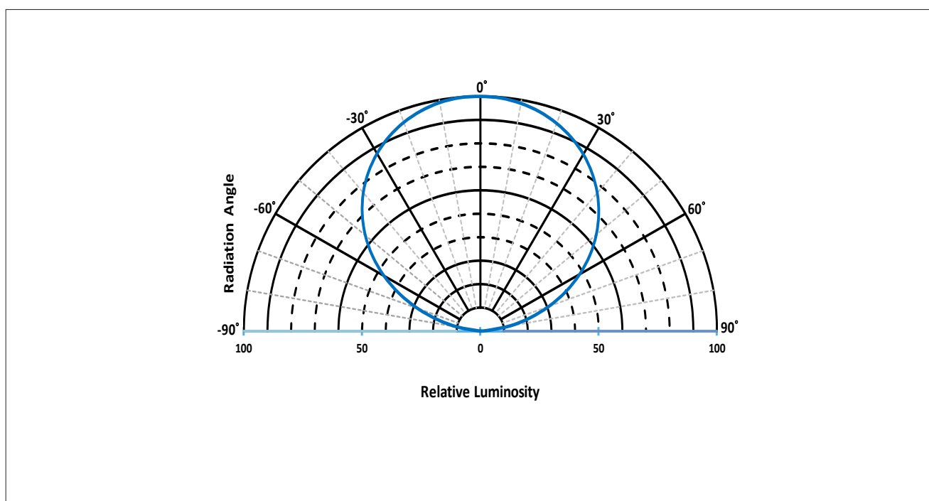
Figure 8: Typical Polar Radiation Pattern at 300mA, T_{sp}=25^{\circ}\text{C}
