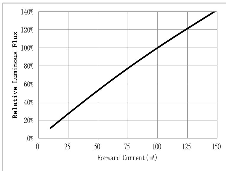
Figure 3: Typical Relative Luminous Flux vs. Forward Current ( T_{sp}=25^{\circ}\text{C} )
