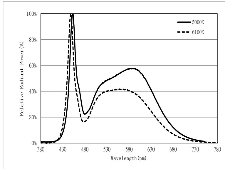
Figure 9: Typical Color Spectrum
