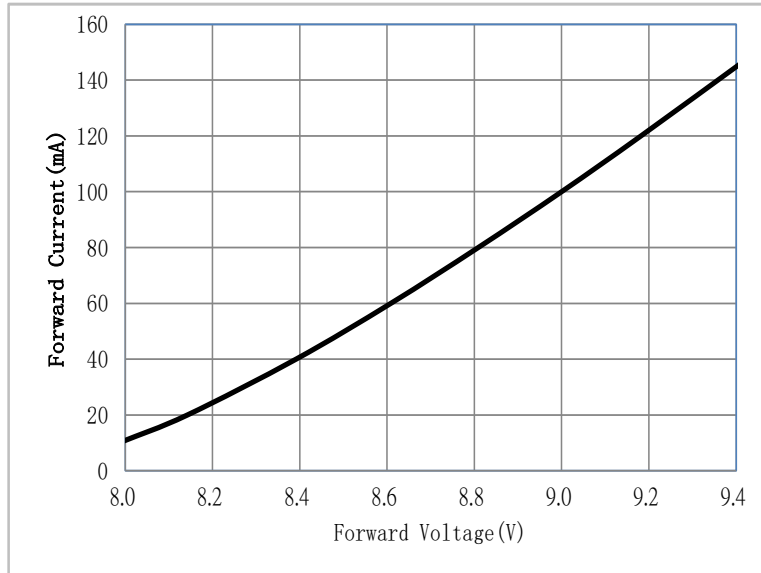
Figure 2: Drive Current vs. Forward Voltage ( T_{sp}=25^{\circ}\text{C} )
