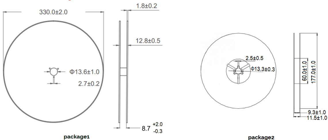
Figure 16: Emitter Reel Drawings
