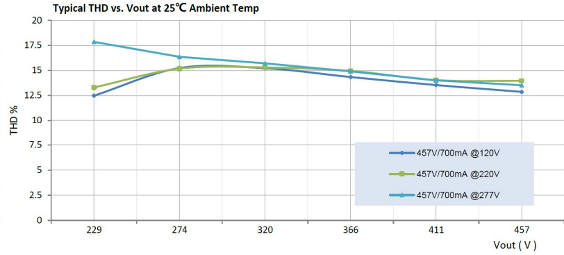
Figure 4: THD vs Output Power
